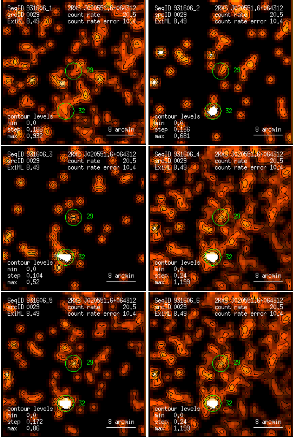
Figure 29: RASS 931606: detection 0029: band rate images, Gaussian filter: (1) PSPC channels 11 – 41, (2) 52 – 90, (3) 91 – 201, (4) 11 – 235, (5) 52 – 201, (6) 11 – 201. Broad band rates in counts/ks. Band rate contour levels in counts/ks/arcmin 2 .
