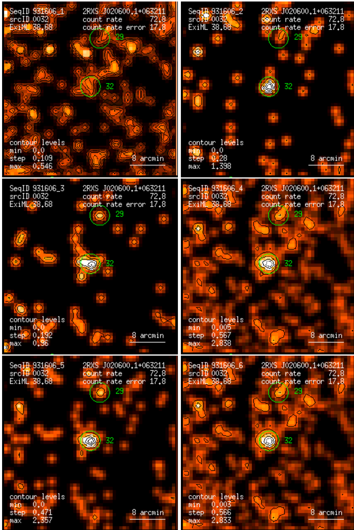
Figure 32: RASS 931606: detection 0032: band rate images, Gaussian filter: (1) PSPC channels 11 – 41, (2) 52 – 90, (3) 91 – 201, (4) 11 – 235, (5) 52 – 201, (6) 11 – 201. Broad band rates in counts/ks. Band rate contour levels in counts/ks/arcmin 2 .
