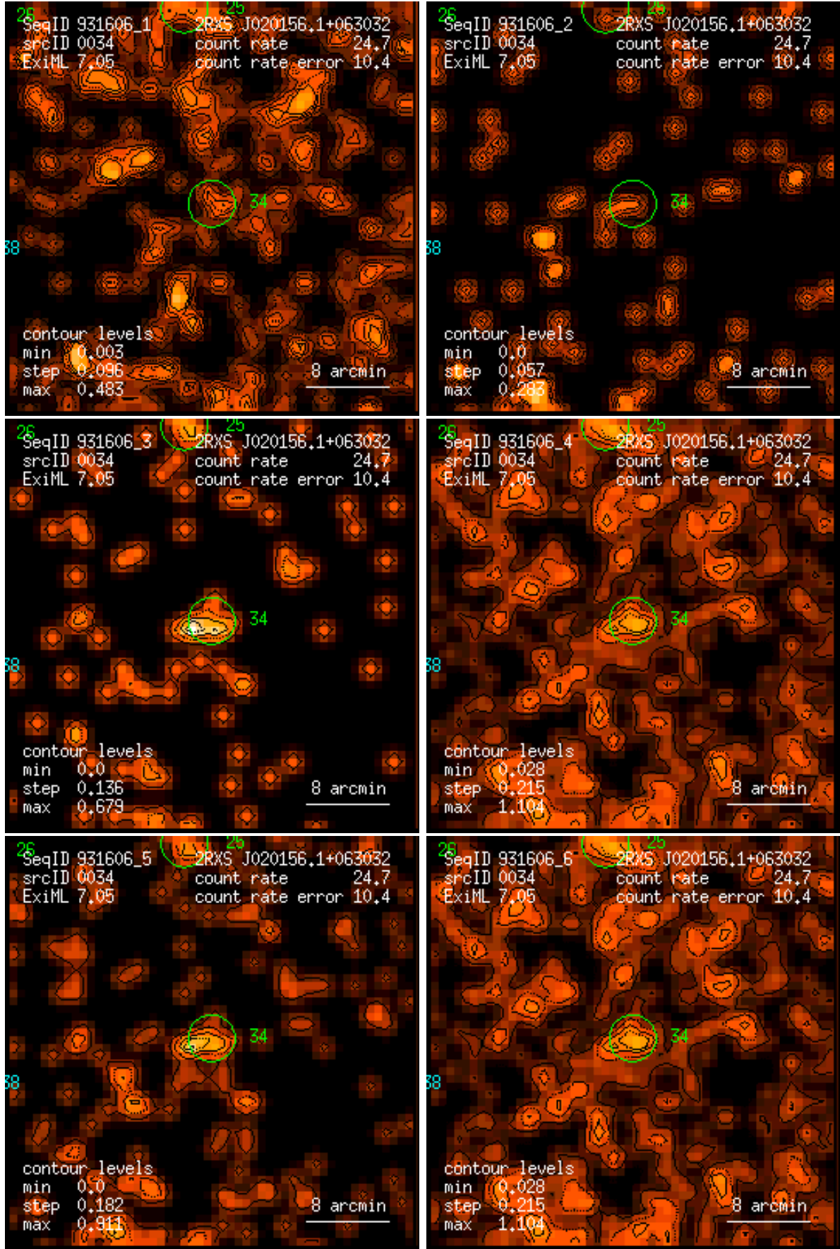
Figure 34: RASS 931606: detection 0034: band rate images, Gaussian filter: (1) PSPC channels 11 – 41, (2) 52 – 90, (3) 91 – 201, (4) 11 – 235, (5) 52 – 201, (6) 11 – 201. Broad band rates in counts/ks. Band rate contour levels in counts/ks/arcmin 2 .
