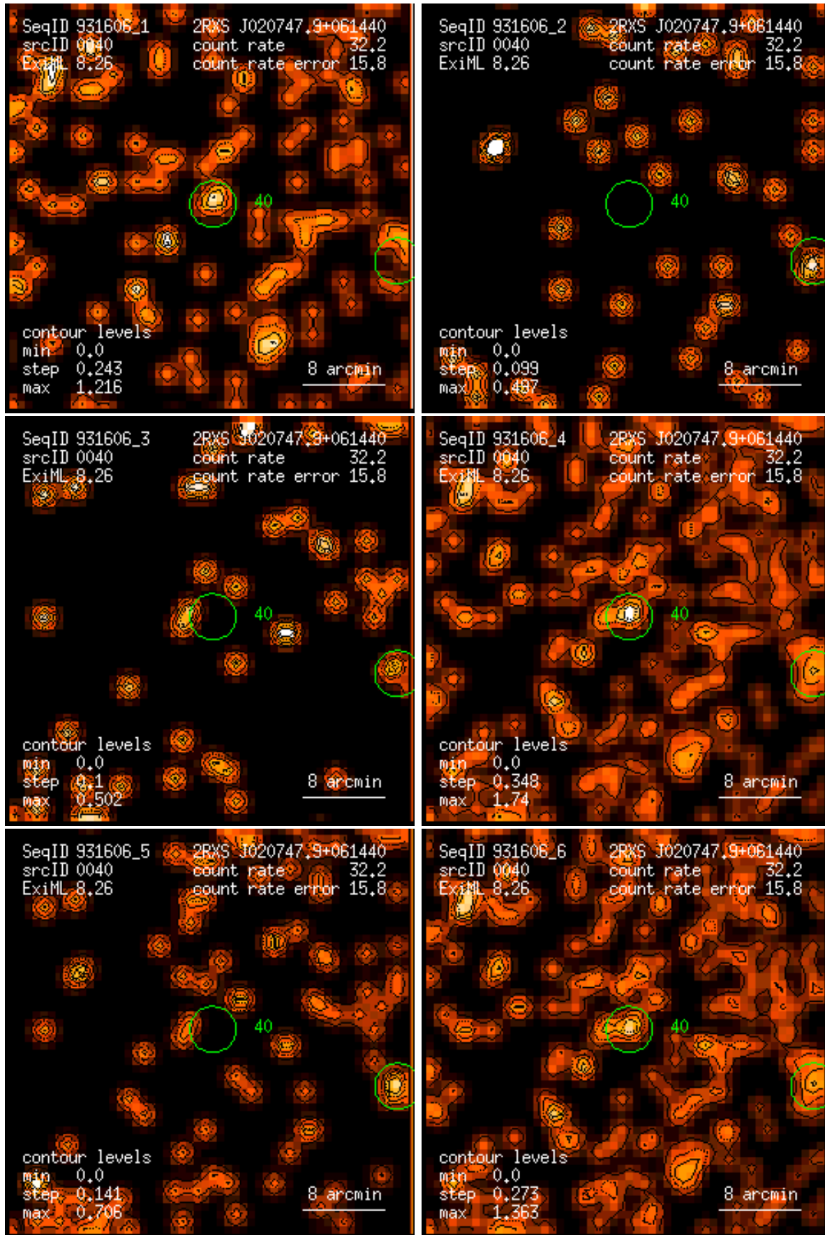
Figure 40: RASS 931606: detection 0040: band rate images, Gaussian filter: (1) PSPC channels 11 – 41, (2) 52 – 90, (3) 91 – 201, (4) 11 – 235, (5) 52 – 201, (6) 11 – 201. Broad band rates in counts/ks. Band rate contour levels in counts/ks/arcmin 2 .
