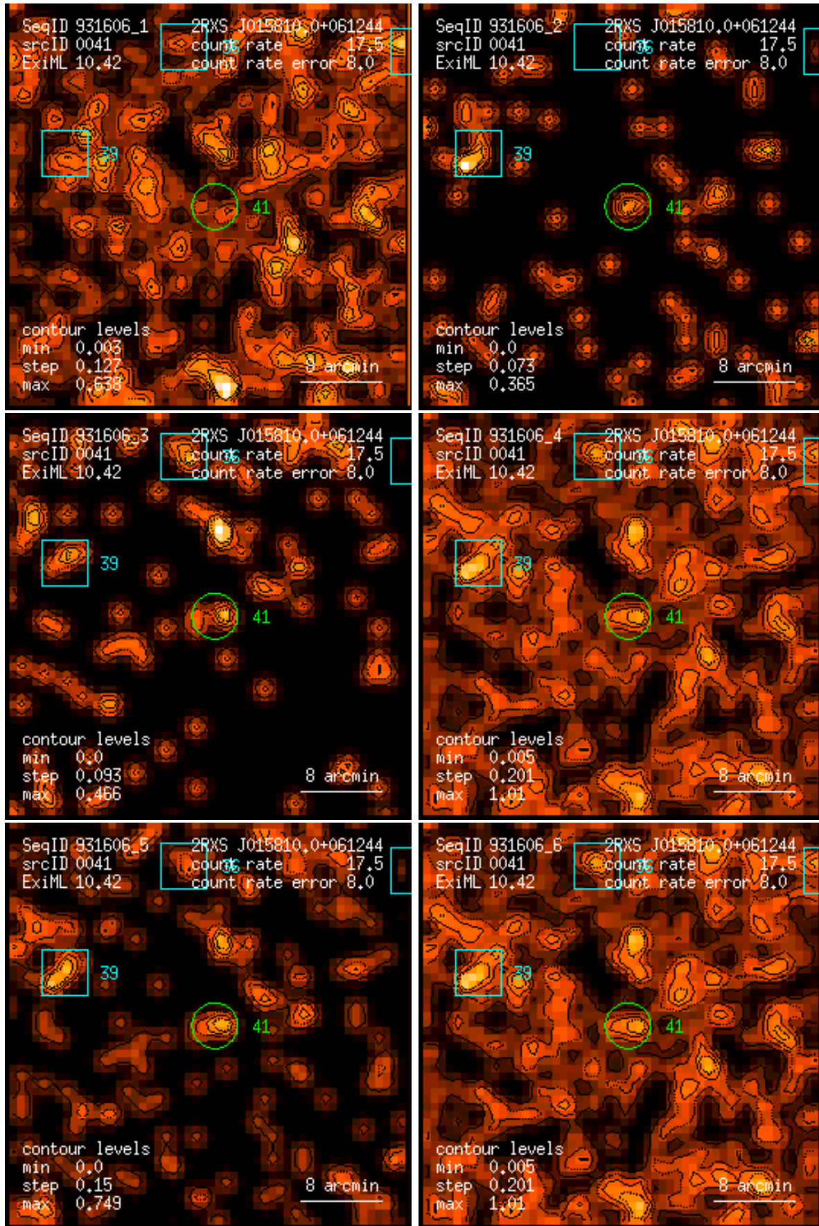
Figure 41: RASS 931606: detection 0041: band rate images, Gaussian filter: (1) PSPC channels 11 – 41, (2) 52 – 90, (3) 91 – 201, (4) 11 – 235, (5) 52 – 201, (6) 11 – 201. Broad band rates in counts/ks. Band rate contour levels in counts/ks/arcmin 2 .
