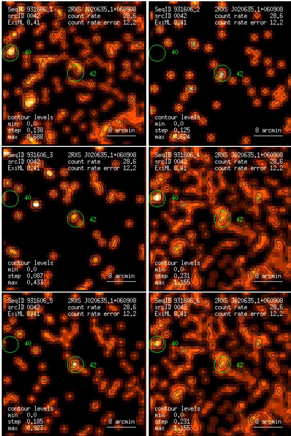
Figure 42: RASS 931606: detection 0042: band rate images, Gaussian filter: (1) PSPC channels 11 – 41, (2) 52 – 90, (3) 91 – 201, (4) 11 – 235, (5) 52 – 201, (6) 11 – 201. Broad band rates in counts/ks. Band rate contour levels in counts/ks/arcmin 2 .
