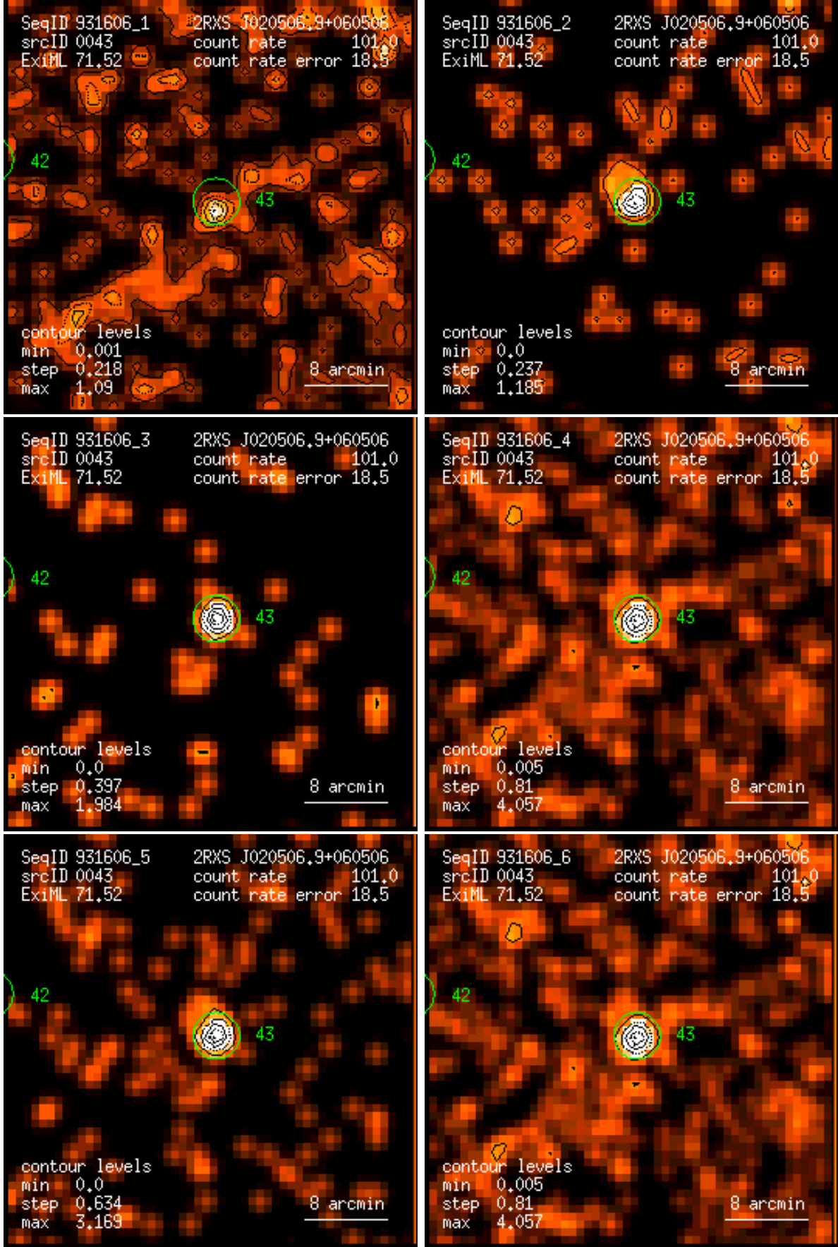
Figure 43: RASS 931606: detection 0043: band rate images, Gaussian filter: (1) PSPC channels 11 – 41, (2) 52 – 90, (3) 91 – 201, (4) 11 – 235, (5) 52 – 201, (6) 11 – 201. Broad band rates in counts/ks. Band rate contour levels in counts/ks/arcmin 2 .
