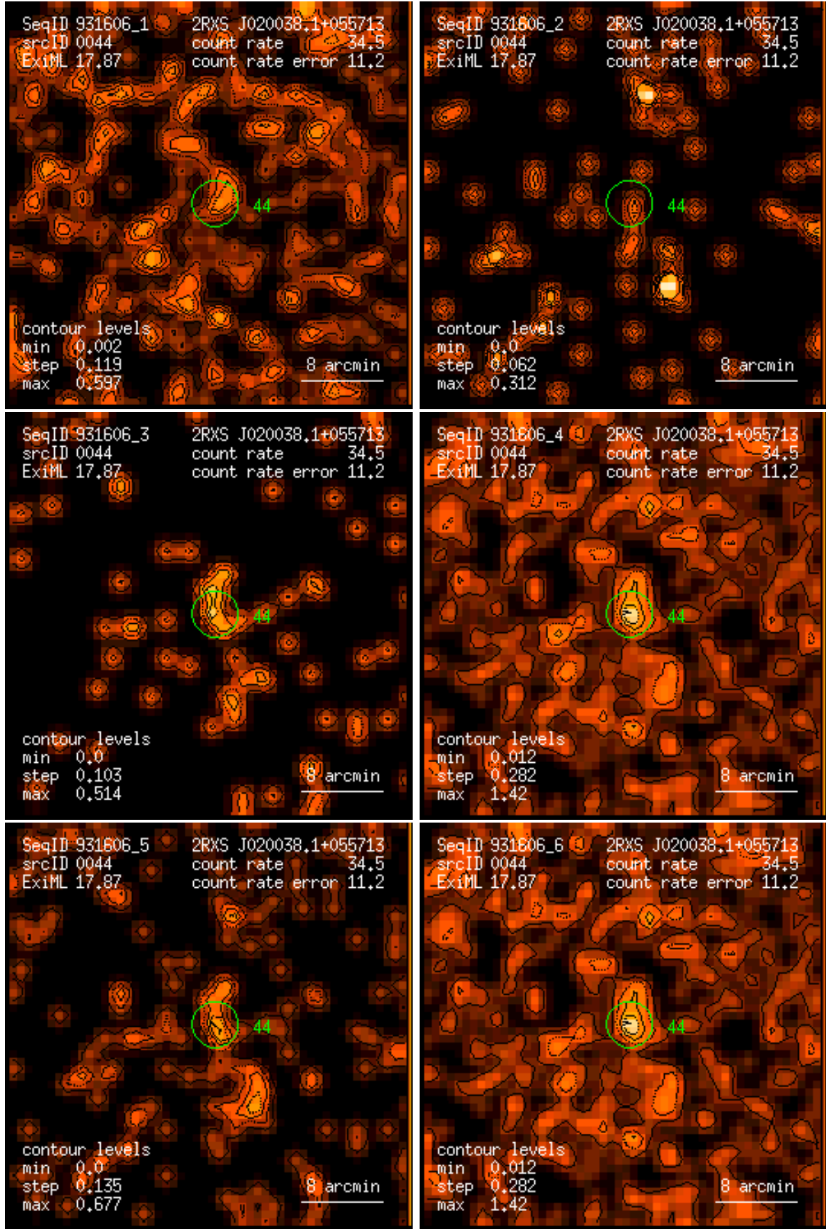
Figure 44: RASS 931606: detection 0044: band rate images, Gaussian filter: (1) PSPC channels 11 – 41, (2) 52 – 90, (3) 91 – 201, (4) 11 – 235, (5) 52 – 201, (6) 11 – 201. Broad band rates in counts/ks. Band rate contour levels in counts/ks/arcmin 2 .
