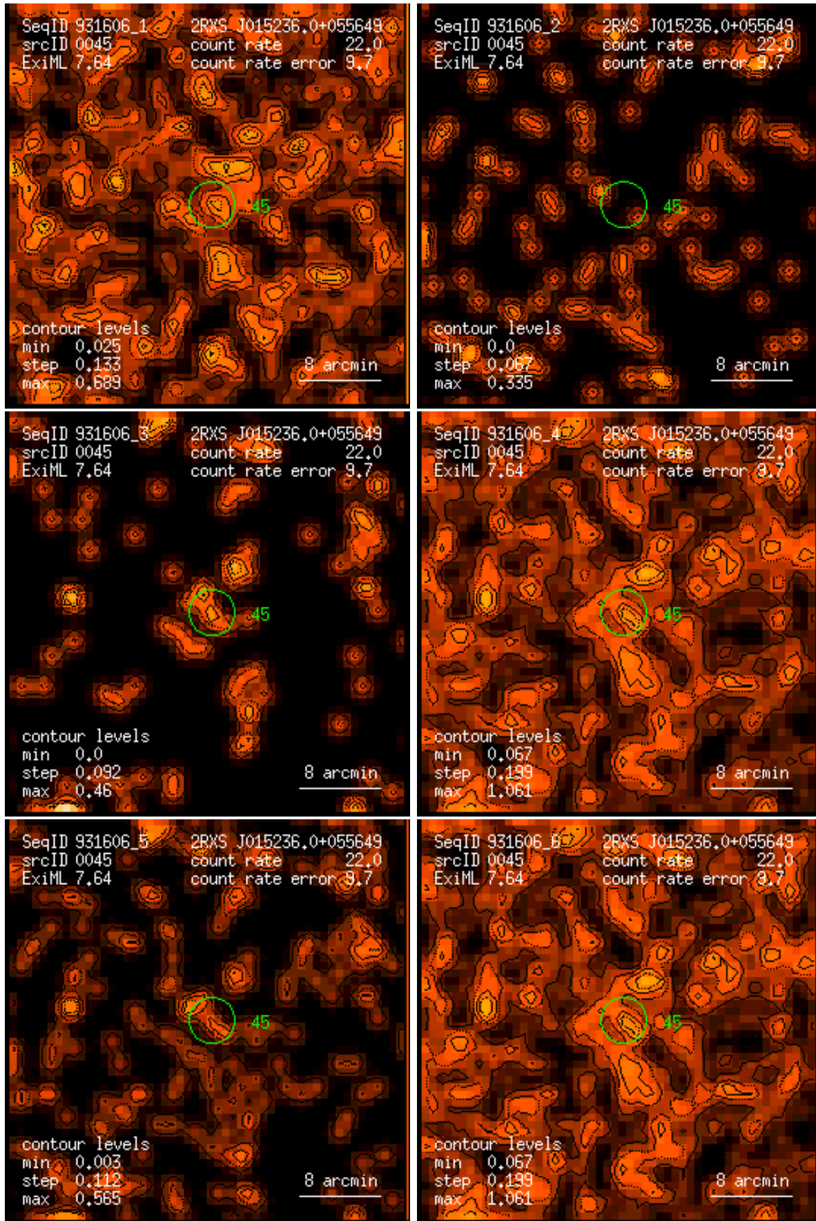
Figure 45: RASS 931606: detection 0045: band rate images, Gaussian filter: (1) PSPC channels 11 – 41, (2) 52 – 90, (3) 91 – 201, (4) 11 – 235, (5) 52 – 201, (6) 11 – 201. Broad band rates in counts/ks. Band rate contour levels in counts/ks/arcmin 2 .
