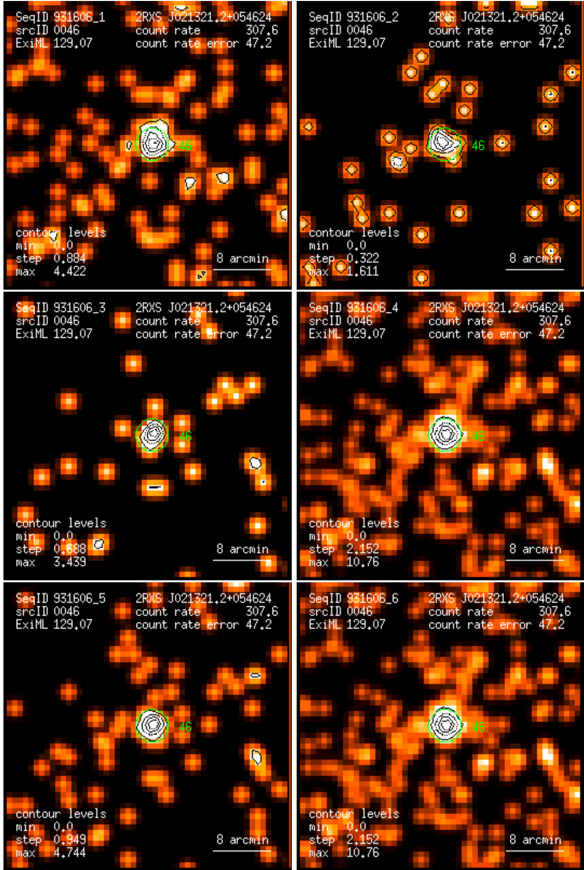
Figure 46: RASS 931606: detection 0046: band rate images, Gaussian filter: (1) PSPC channels 11 – 41, (2) 52 – 90, (3) 91 – 201, (4) 11 – 235, (5) 52 – 201, (6) 11 – 201. Broad band rates in counts/ks. Band rate contour levels in counts/ks/arcmin 2 .
