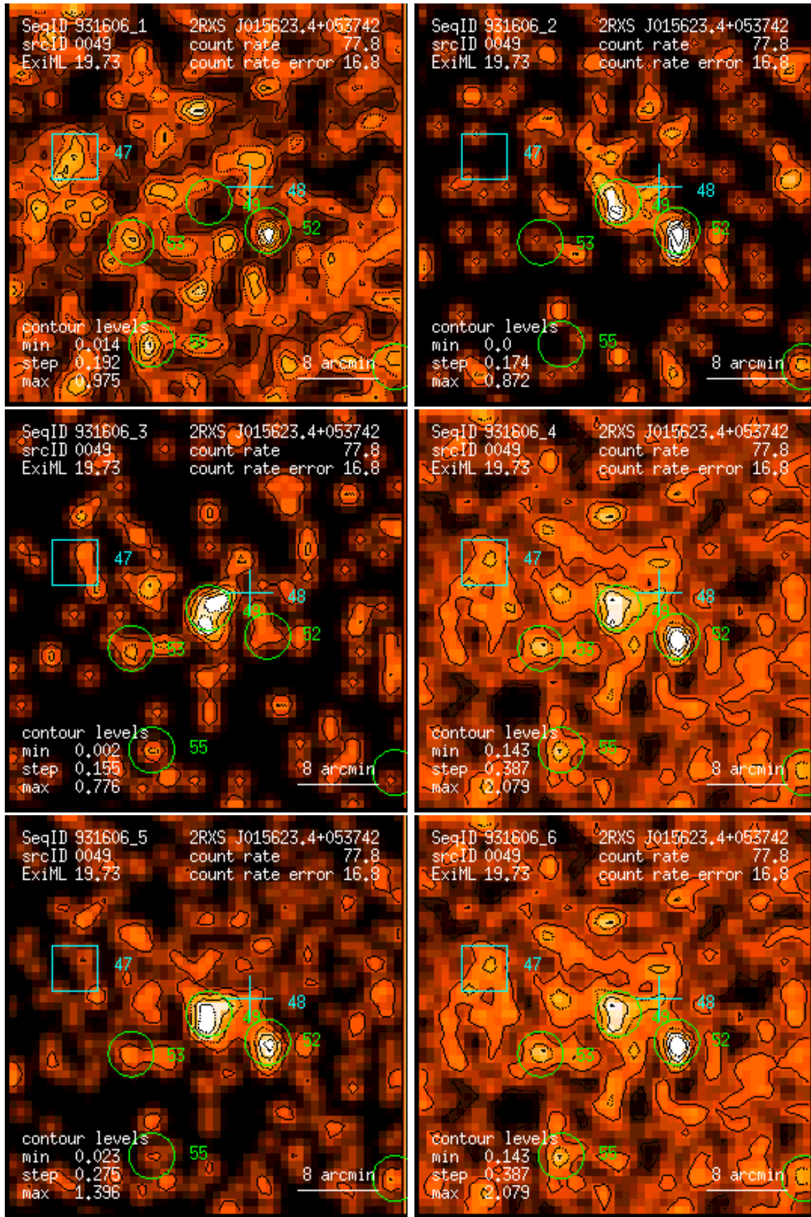
Figure 49: RASS 931606: detection 0049: band rate images, Gaussian filter: (1) PSPC channels 11 – 41, (2) 52 – 90, (3) 91 – 201, (4) 11 – 235, (5) 52 – 201, (6) 11 – 201. Broad band rates in counts/ks. Band rate contour levels in counts/ks/arcmin 2 .
