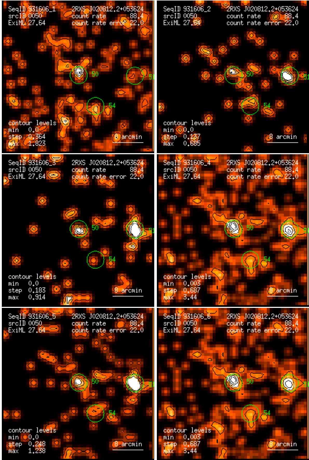
Figure 50: RASS 931606: detection 0050: band rate images, Gaussian filter: (1) PSPC channels 11 – 41, (2) 52 – 90, (3) 91 – 201, (4) 11 – 235, (5) 52 – 201, (6) 11 – 201. Broad band rates in counts/ks. Band rate contour levels in counts/ks/arcmin 2 .
