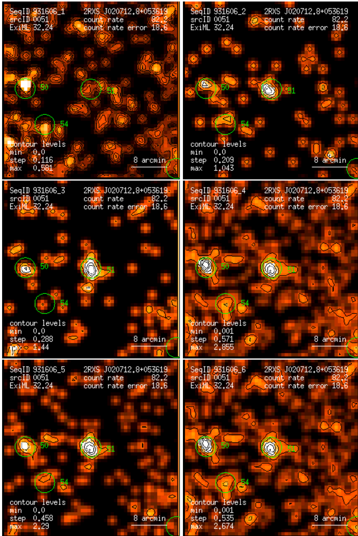
Figure 51: RASS 931606: detection 0051: band rate images, Gaussian filter: (1) PSPC channels 11 – 41, (2) 52 – 90, (3) 91 – 201, (4) 11 – 235, (5) 52 – 201, (6) 11 – 201. Broad band rates in counts/ks. Band rate contour levels in counts/ks/arcmin 2 .
