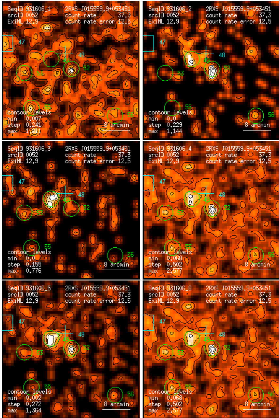
Figure 52: RASS 931606: detection 0052: band rate images, Gaussian filter: (1) PSPC channels 11 – 41, (2) 52 – 90, (3) 91 – 201, (4) 11 – 235, (5) 52 – 201, (6) 11 – 201. Broad band rates in counts/ks. Band rate contour levels in counts/ks/arcmin 2 .
