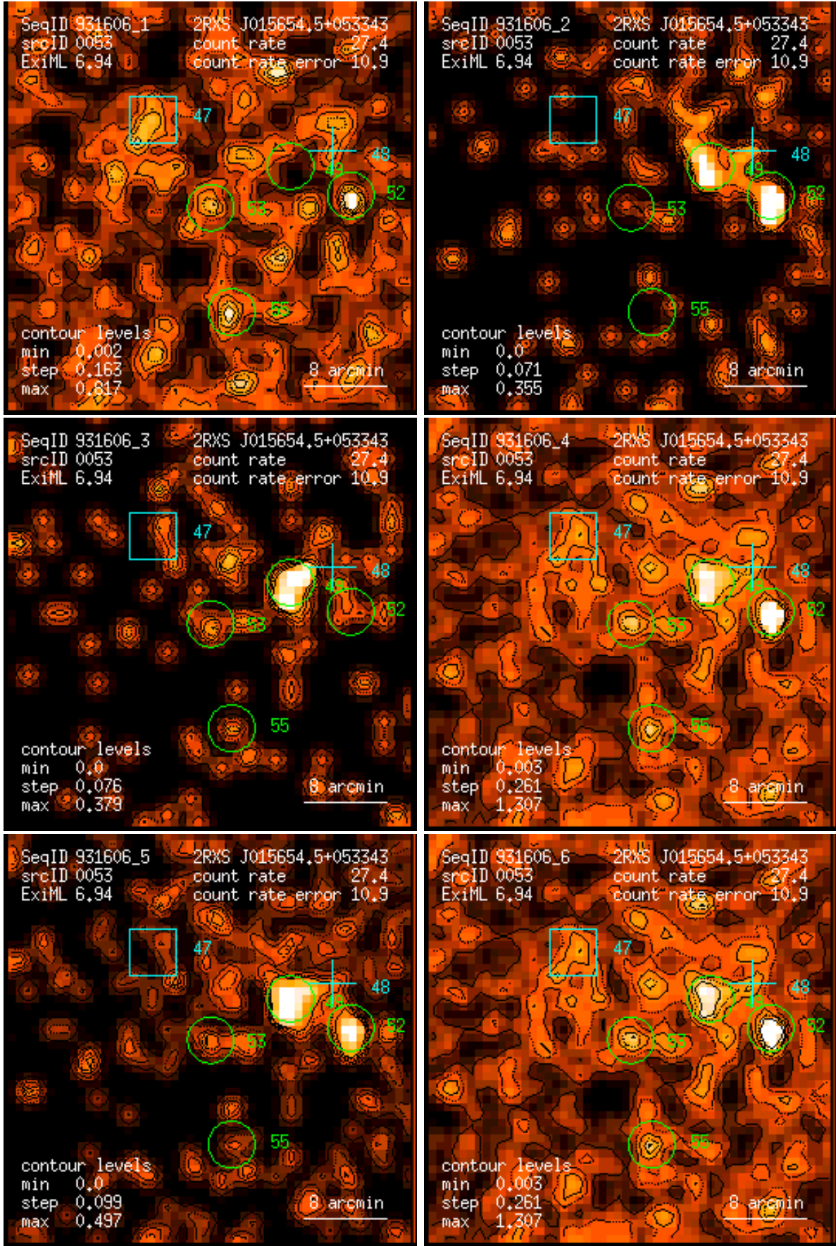
Figure 53: RASS 931606: detection 0053: band rate images, Gaussian filter: (1) PSPC channels 11 – 41, (2) 52 – 90, (3) 91 – 201, (4) 11 – 235, (5) 52 – 201, (6) 11 – 201. Broad band rates in counts/ks. Band rate contour levels in counts/ks/arcmin 2 .
