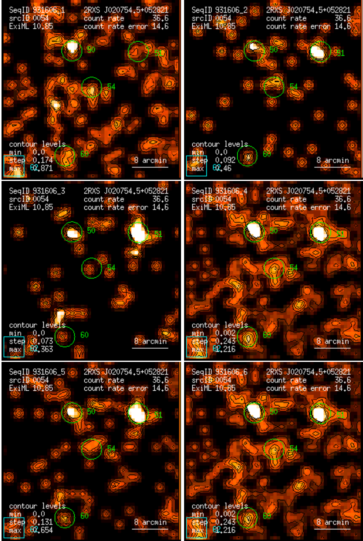
Figure 54: RASS 931606: detection 0054: band rate images, Gaussian filter: (1) PSPC channels 11 – 41, (2) 52 – 90, (3) 91 – 201, (4) 11 – 235, (5) 52 – 201, (6) 11 – 201. Broad band rates in counts/ks. Band rate contour levels in counts/ks/arcmin 2 .
