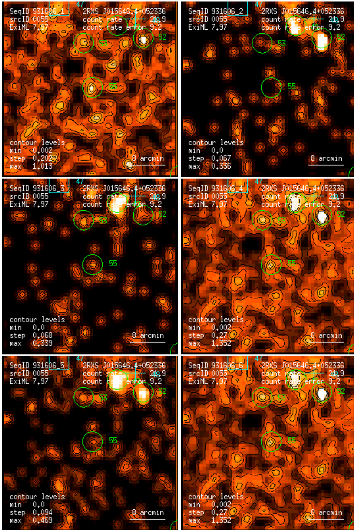
Figure 55: RASS 931606: detection 0055: band rate images, Gaussian filter: (1) PSPC channels 11 – 41, (2) 52 – 90, (3) 91 – 201, (4) 11 – 235, (5) 52 – 201, (6) 11 – 201. Broad band rates in counts/ks. Band rate contour levels in counts/ks/arcmin 2 .
