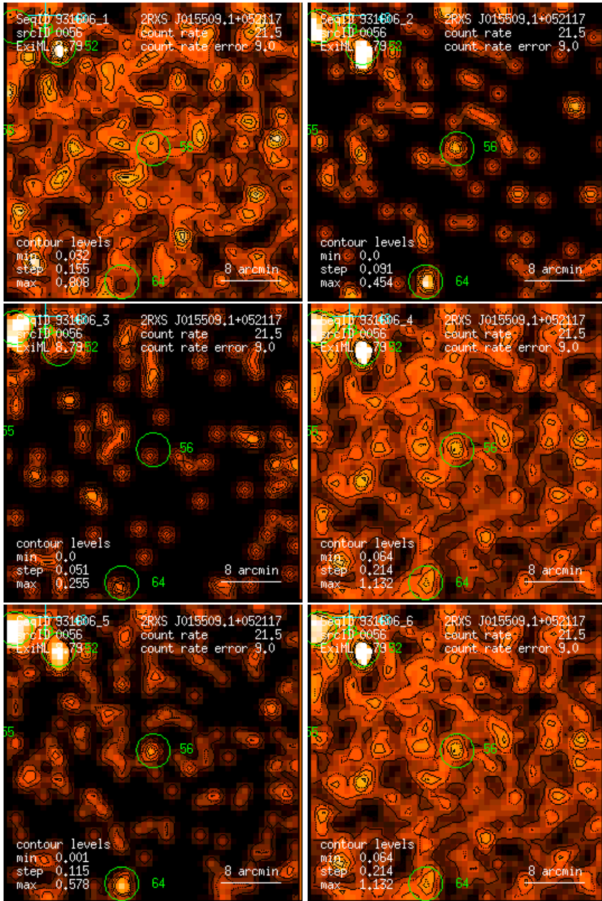
Figure 56: RASS 931606: detection 0056: band rate images, Gaussian filter: (1) PSPC channels 11 – 41, (2) 52 – 90, (3) 91 – 201, (4) 11 – 235, (5) 52 – 201, (6) 11 – 201. Broad band rates in counts/ks. Band rate contour levels in counts/ks/arcmin 2 .
