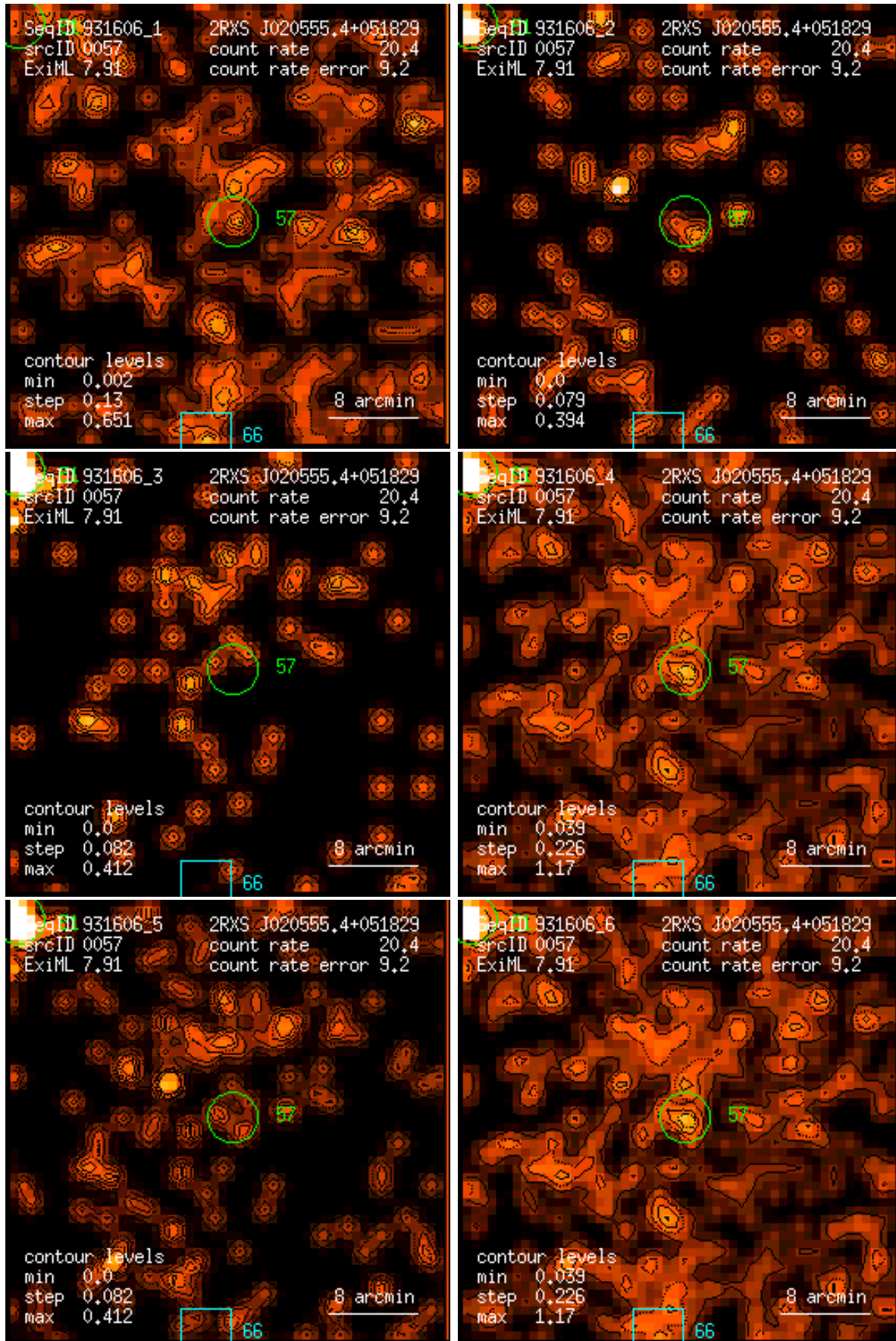
Figure 57: RASS 931606: detection 0057: band rate images, Gaussian filter: (1) PSPC channels 11 – 41, (2) 52 – 90, (3) 91 – 201, (4) 11 – 235, (5) 52 – 201, (6) 11 – 201. Broad band rates in counts/ks. Band rate contour levels in counts/ks/arcmin 2 .
