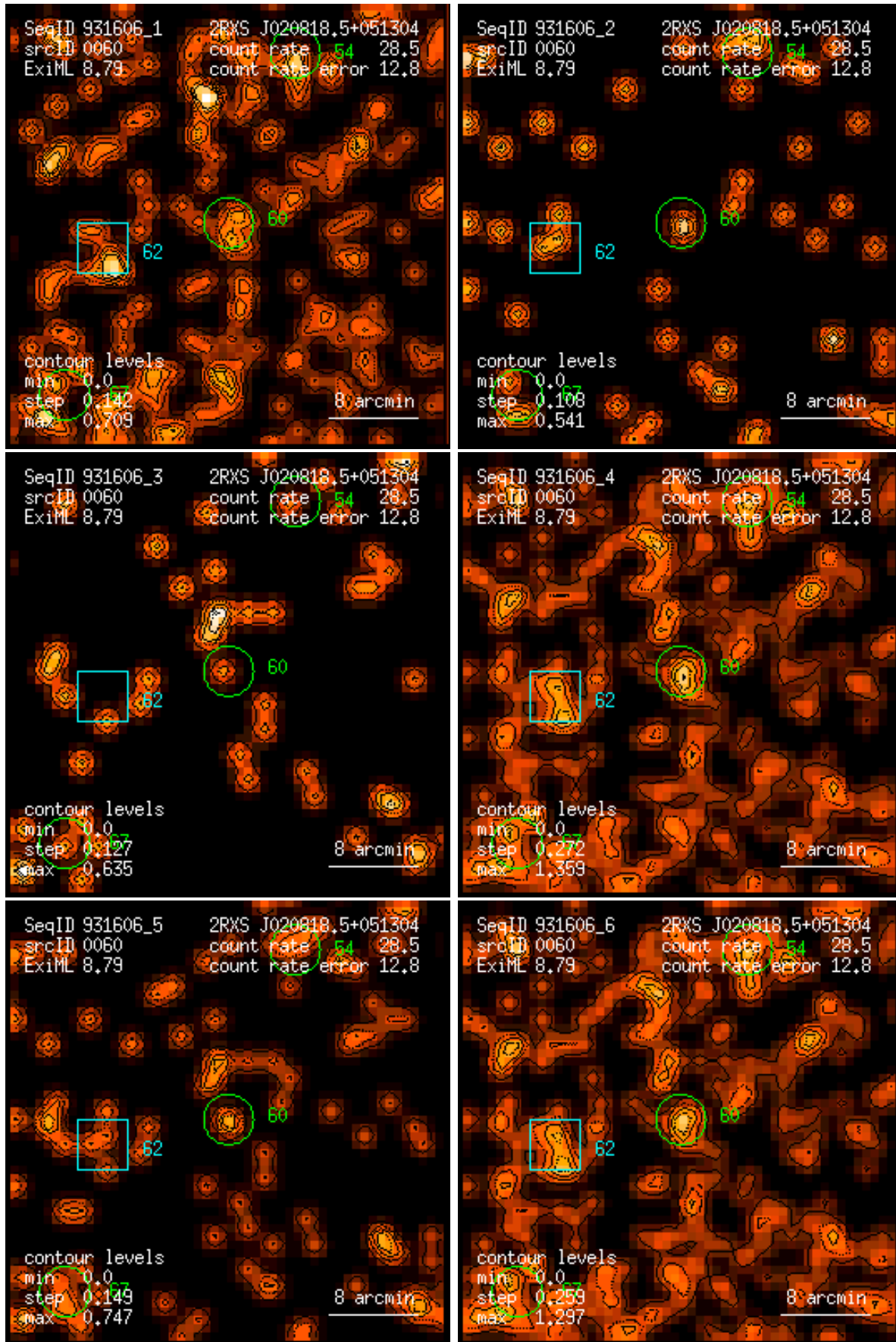
Figure 60: RASS 931606: detection 0060: band rate images, Gaussian filter: (1) PSPC channels 11 – 41, (2) 52 – 90, (3) 91 – 201, (4) 11 – 235, (5) 52 – 201, (6) 11 – 201. Broad band rates in counts/ks. Band rate contour levels in counts/ks/arcmin 2 .
