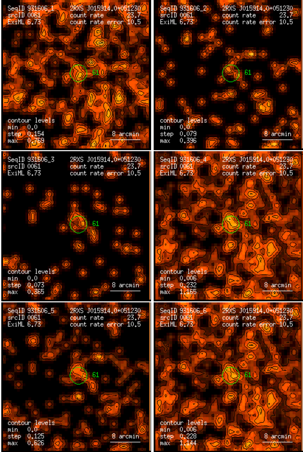
Figure 61: RASS 931606: detection 0061: band rate images, Gaussian filter: (1) PSPC channels 11 – 41, (2) 52 – 90, (3) 91 – 201, (4) 11 – 235, (5) 52 – 201, (6) 11 – 201. Broad band rates in counts/ks. Band rate contour levels in counts/ks/arcmin 2 .
