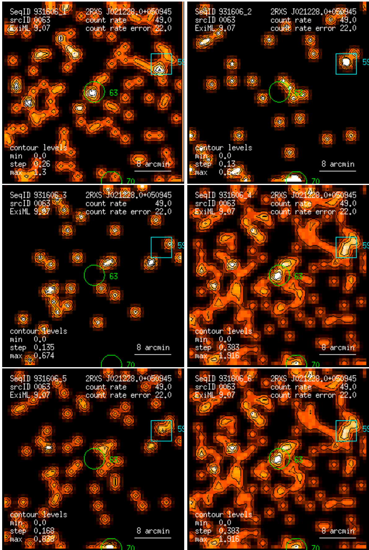
Figure 63: RASS 931606: detection 0063: band rate images, Gaussian filter: (1) PSPC channels 11 – 41, (2) 52 – 90, (3) 91 – 201, (4) 11 – 235, (5) 52 – 201, (6) 11 – 201. Broad band rates in counts/ks. Band rate contour levels in counts/ks/arcmin 2 .
