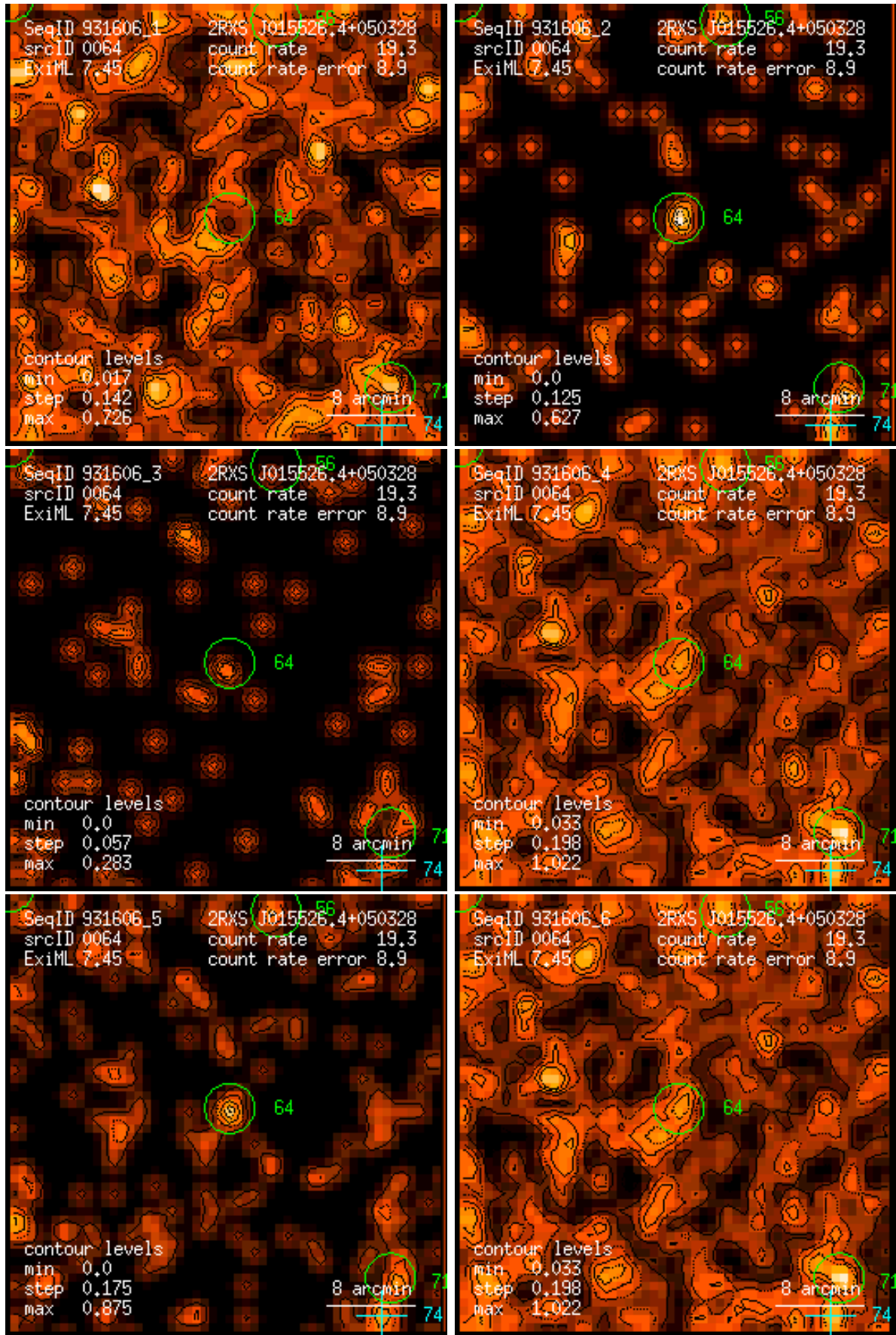
Figure 64: RASS 931606: detection 0064: band rate images, Gaussian filter: (1) PSPC channels 11 – 41, (2) 52 – 90, (3) 91 – 201, (4) 11 – 235, (5) 52 – 201, (6) 11 – 201. Broad band rates in counts/ks. Band rate contour levels in counts/ks/arcmin 2 .
