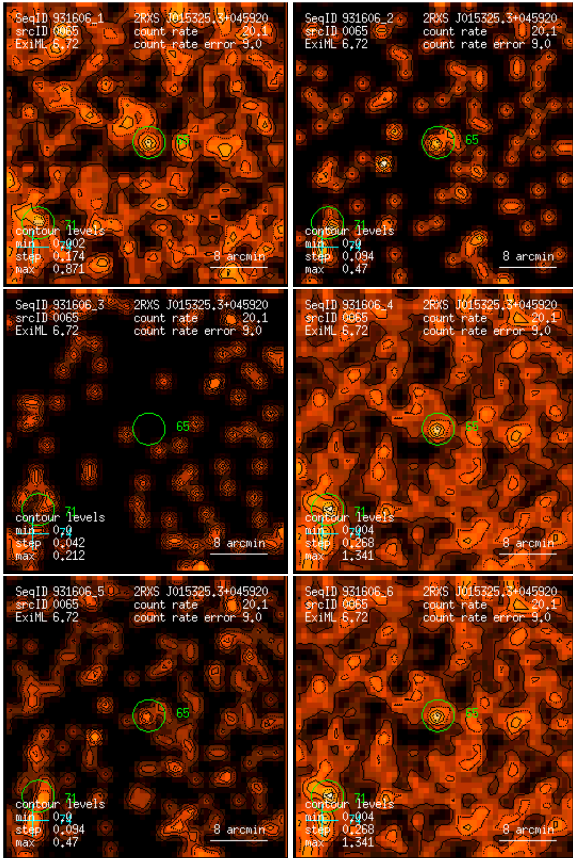
Figure 65: RASS 931606: detection 0065: band rate images, Gaussian filter: (1) PSPC channels 11 – 41, (2) 52 – 90, (3) 91 – 201, (4) 11 – 235, (5) 52 – 201, (6) 11 – 201. Broad band rates in counts/ks. Band rate contour levels in counts/ks/arcmin 2 .
