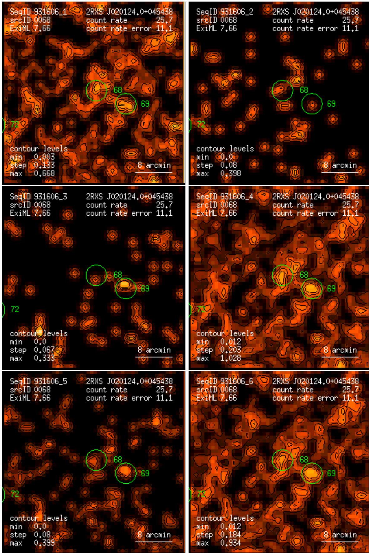
Figure 68: RASS 931606: detection 0068: band rate images, Gaussian filter: (1) PSPC channels 11 – 41, (2) 52 – 90, (3) 91 – 201, (4) 11 – 235, (5) 52 – 201, (6) 11 – 201. Broad band rates in counts/ks. Band rate contour levels in counts/ks/arcmin 2 .
