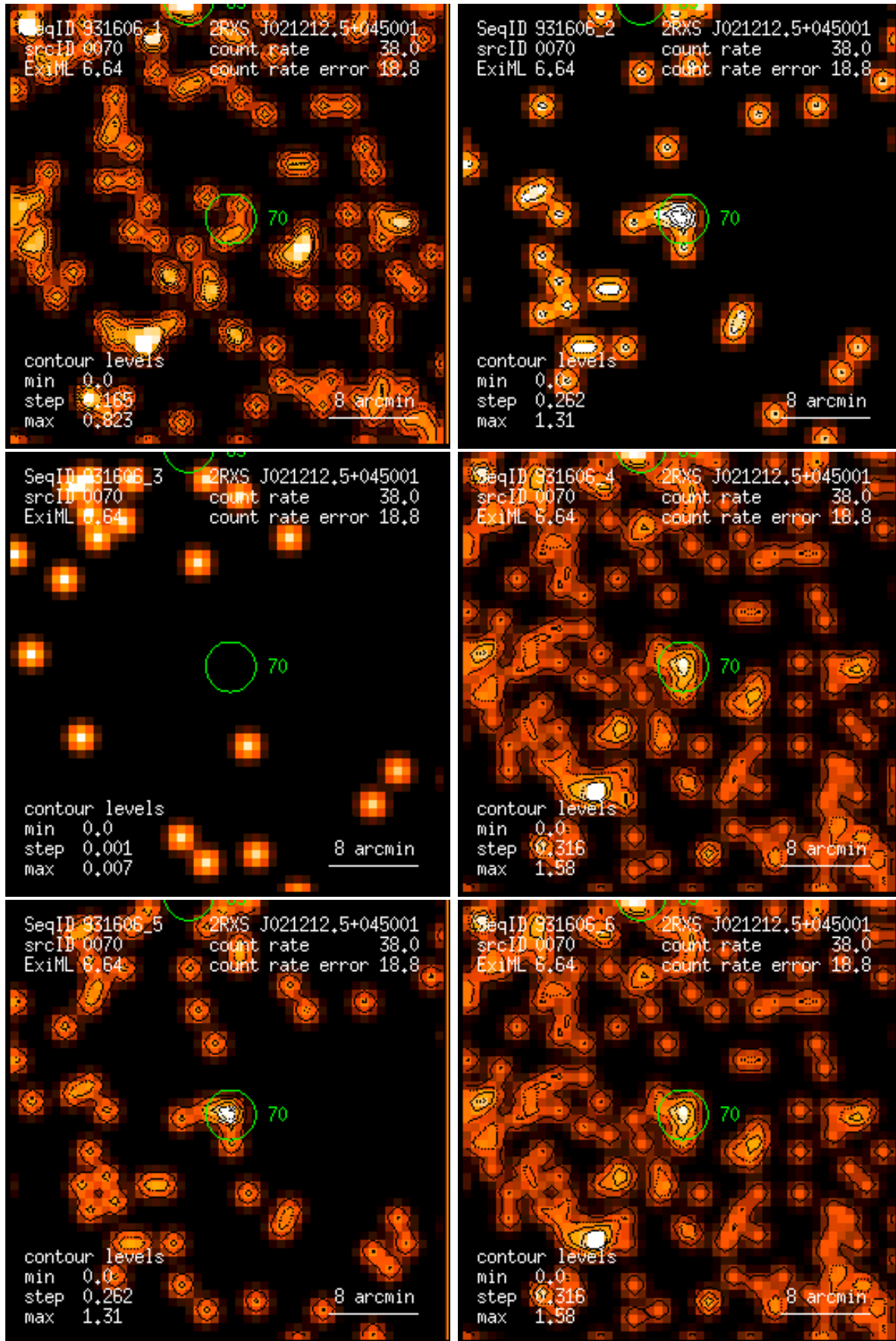
Figure 70: RASS 931606: detection 0070: band rate images, Gaussian filter: (1) PSPC channels 11 – 41, (2) 52 – 90, (3) 91 – 201, (4) 11 – 235, (5) 52 – 201, (6) 11 – 201. Broad band rates in counts/ks. Band rate contour levels in counts/ks/arcmin 2 .
