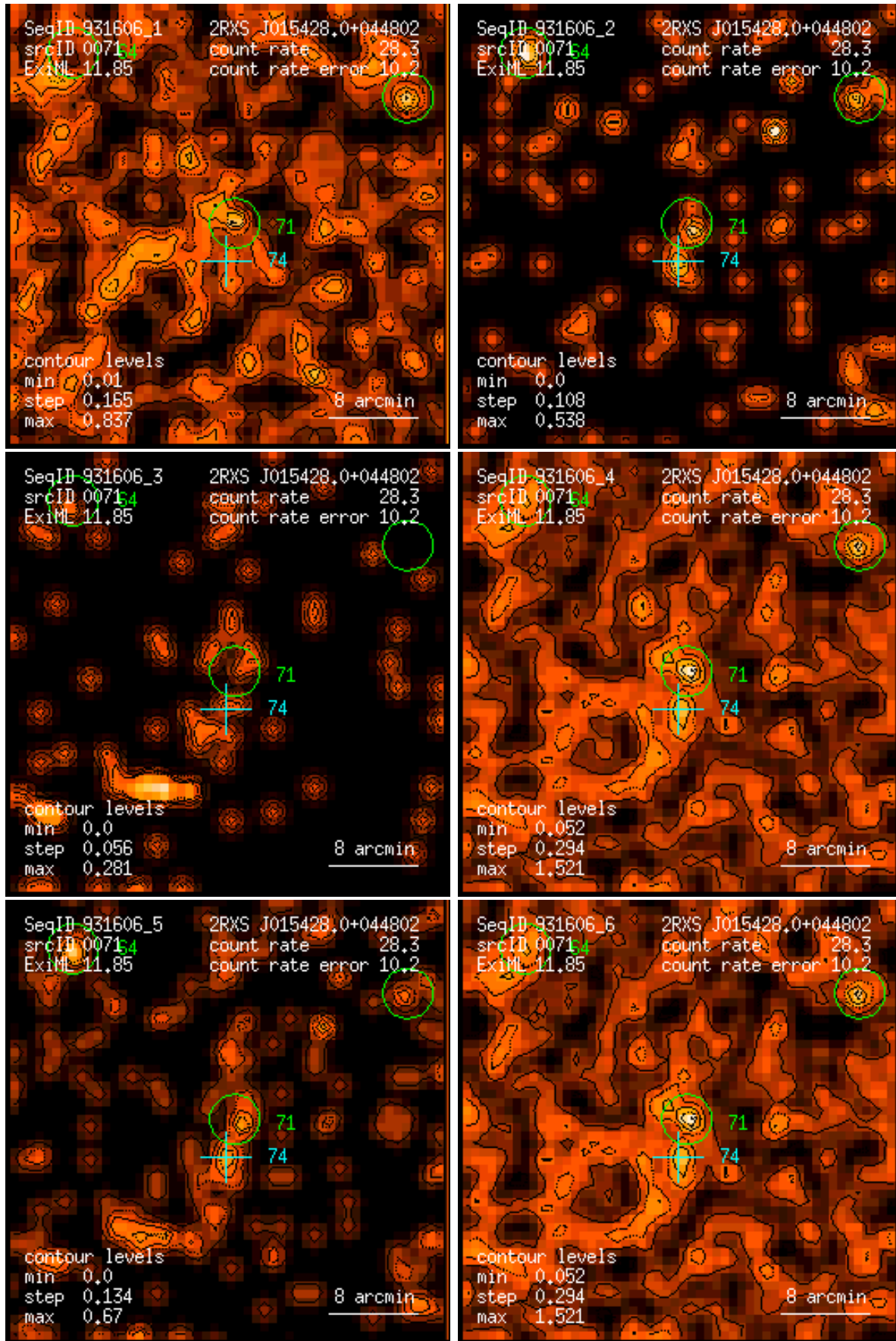
Figure 71: RASS 931606: detection 0071: band rate images, Gaussian filter: (1) PSPC channels 11 – 41, (2) 52 – 90, (3) 91 – 201, (4) 11 – 235, (5) 52 – 201, (6) 11 – 201. Broad band rates in counts/ks. Band rate contour levels in counts/ks/arcmin 2 .
