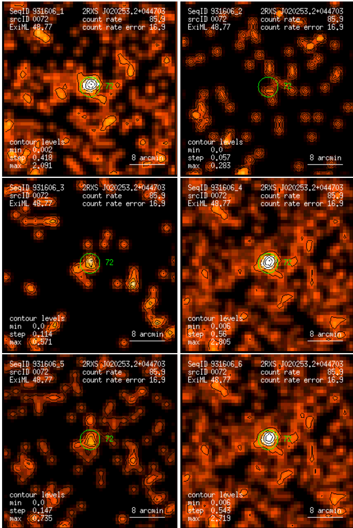
Figure 72: RASS 931606: detection 0072: band rate images, Gaussian filter: (1) PSPC channels 11 – 41, (2) 52 – 90, (3) 91 – 201, (4) 11 – 235, (5) 52 – 201, (6) 11 – 201. Broad band rates in counts/ks. Band rate contour levels in counts/ks/arcmin 2 .
