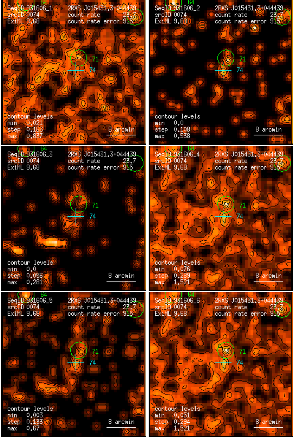
Figure 74: RASS 931606: detection 0074: band rate images, Gaussian filter: (1) PSPC channels 11 – 41, (2) 52 – 90, (3) 91 – 201, (4) 11 – 235, (5) 52 – 201, (6) 11 – 201. Broad band rates in counts/ks. Band rate contour levels in counts/ks/arcmin 2 .
