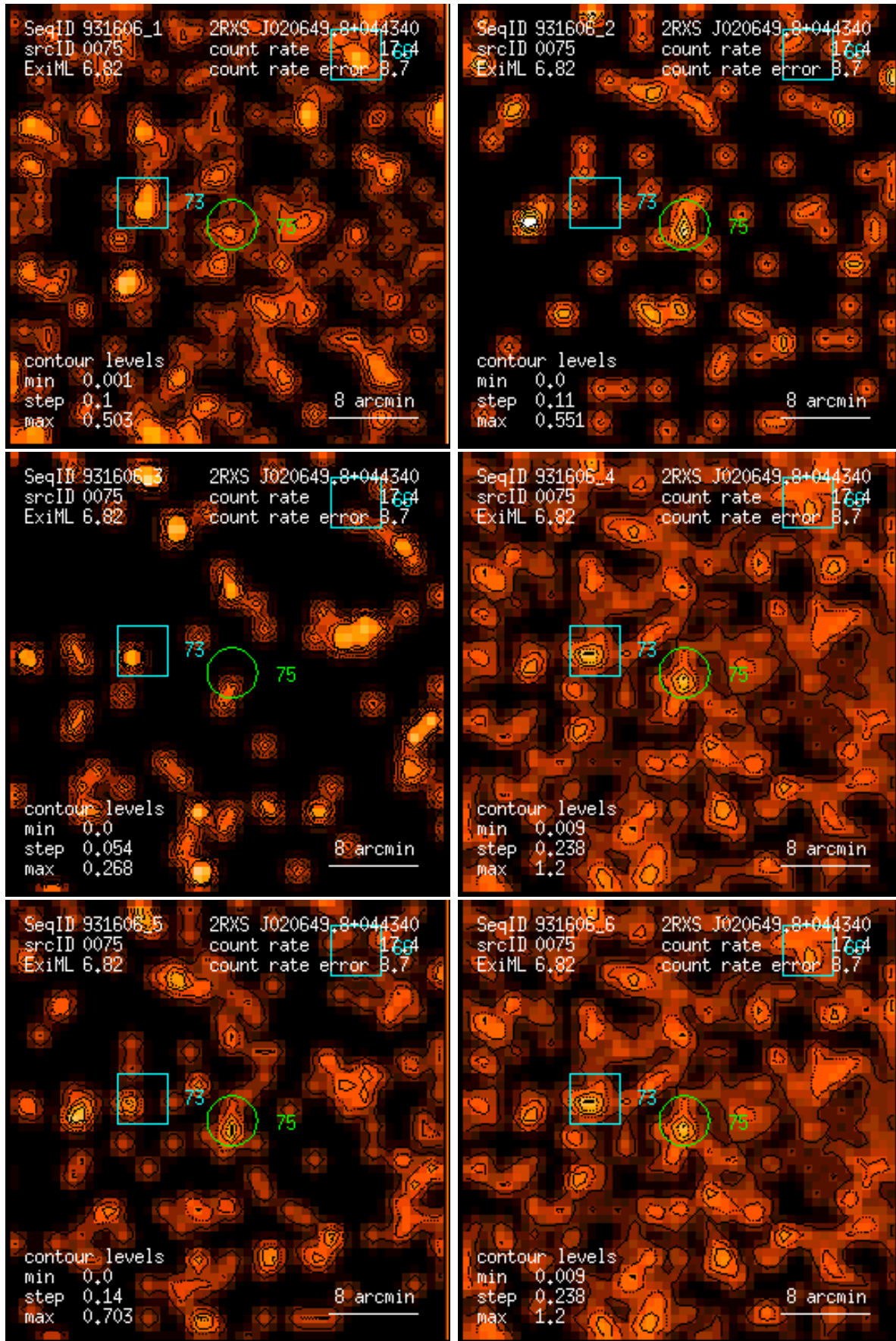
Figure 75: RASS 931606: detection 0075: band rate images, Gaussian filter: (1) PSPC channels 11 – 41, (2) 52 – 90, (3) 91 – 201, (4) 11 – 235, (5) 52 – 201, (6) 11 – 201. Broad band rates in counts/ks. Band rate contour levels in counts/ks/arcmin 2 .
