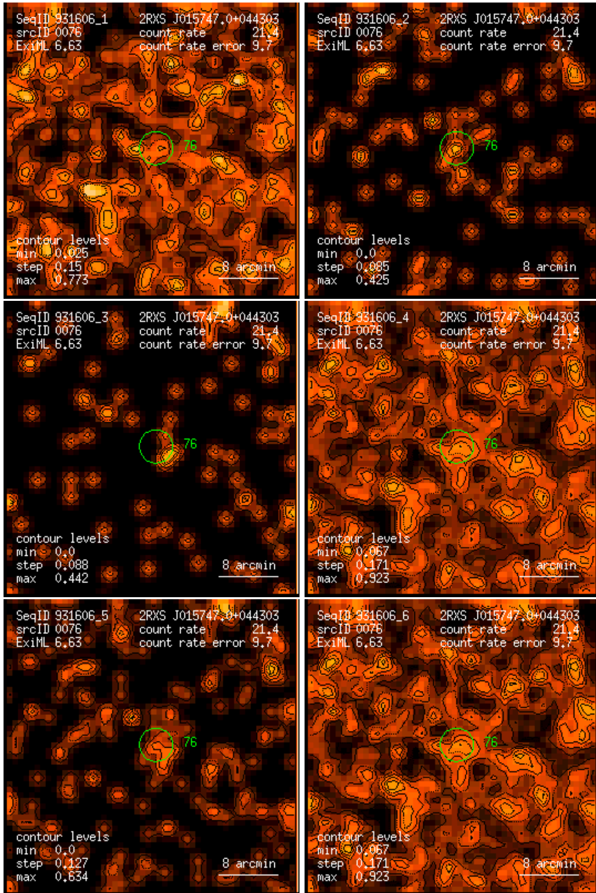
Figure 76: RASS 931606: detection 0076: band rate images, Gaussian filter: (1) PSPC channels 11 – 41, (2) 52 – 90, (3) 91 – 201, (4) 11 – 235, (5) 52 – 201, (6) 11 – 201. Broad band rates in counts/ks. Band rate contour levels in counts/ks/arcmin 2 .
