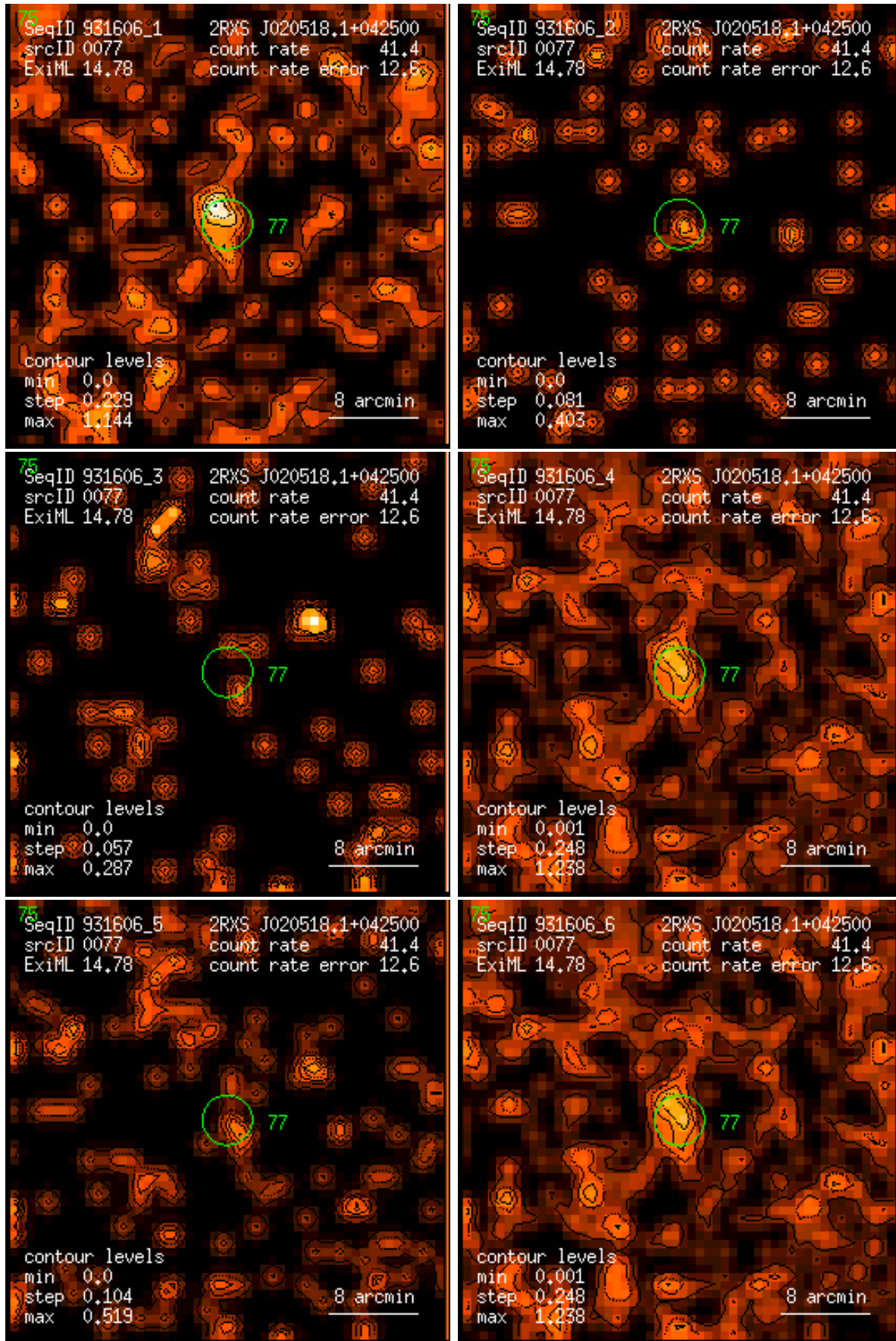
Figure 77: RASS 931606: detection 0077: band rate images, Gaussian filter: (1) PSPC channels 11 – 41, (2) 52 – 90, (3) 91 – 201, (4) 11 – 235, (5) 52 – 201, (6) 11 – 201. Broad band rates in counts/ks. Band rate contour levels in counts/ks/arcmin 2 .
