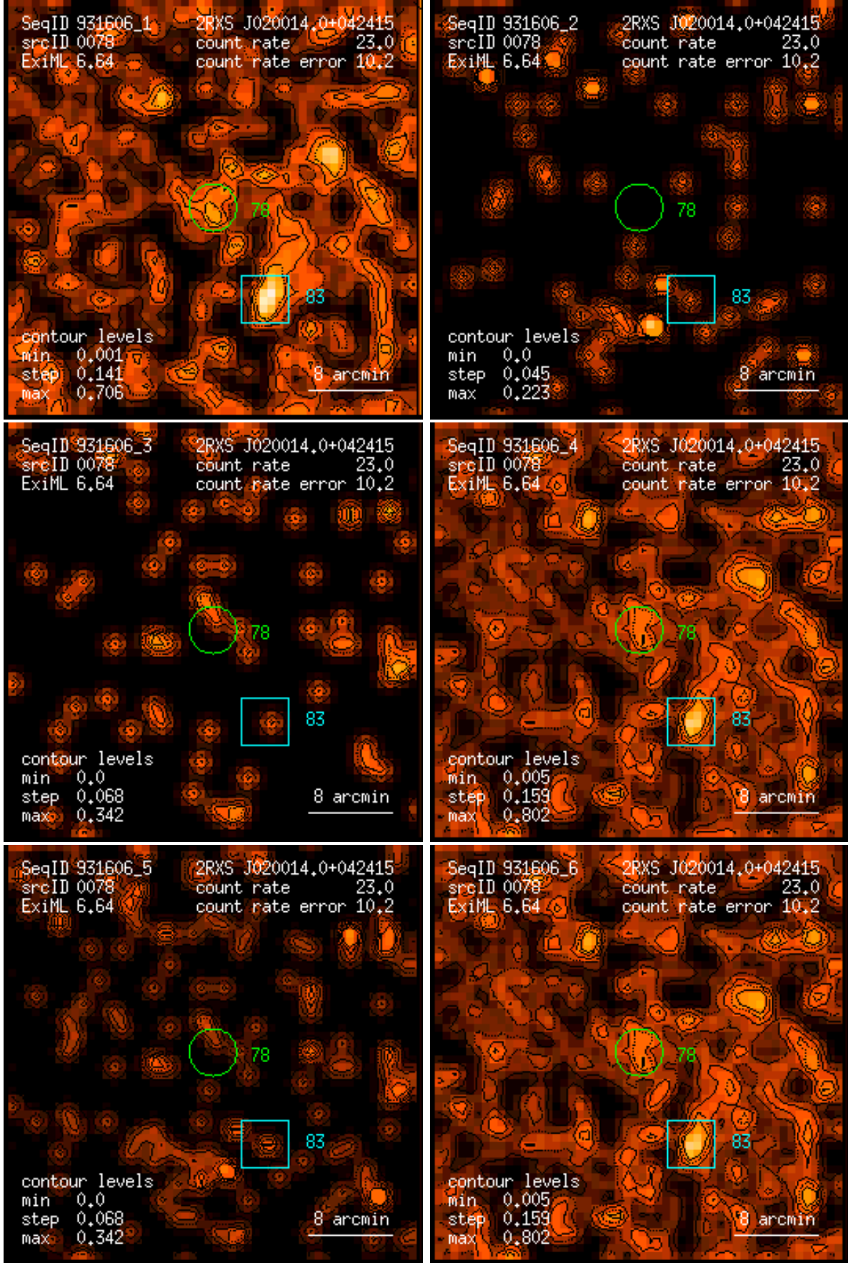
Figure 78: RASS 931606: detection 0078: band rate images, Gaussian filter: (1) PSPC channels 11 – 41, (2) 52 – 90, (3) 91 – 201, (4) 11 – 235, (5) 52 – 201, (6) 11 – 201. Broad band rates in counts/ks. Band rate contour levels in counts/ks/arcmin 2 .
