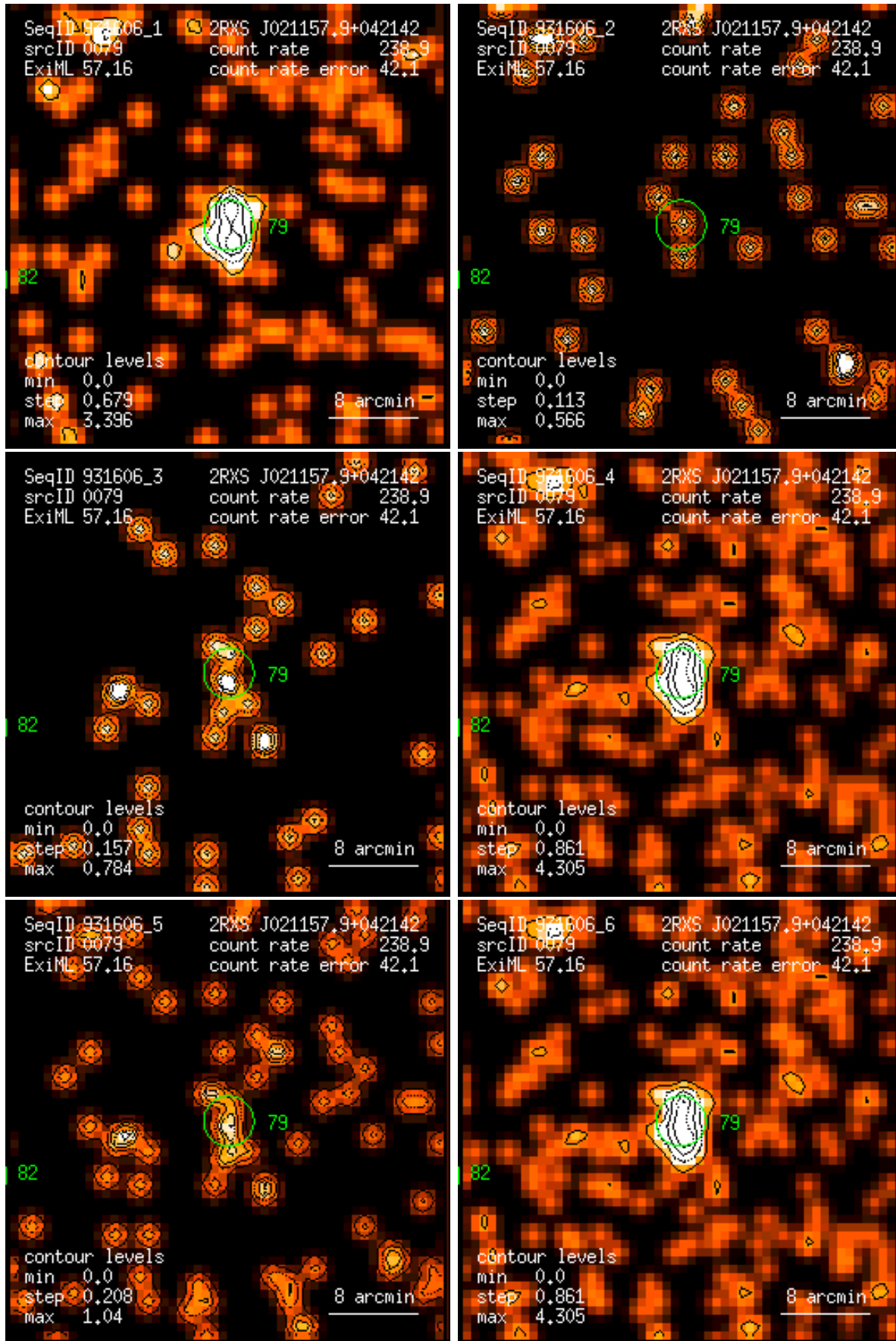
Figure 79: RASS 931606: detection 0079: band rate images, Gaussian filter: (1) PSPC channels 11 – 41, (2) 52 – 90, (3) 91 – 201, (4) 11 – 235, (5) 52 – 201, (6) 11 – 201. Broad band rates in counts/ks. Band rate contour levels in counts/ks/arcmin 2 .
