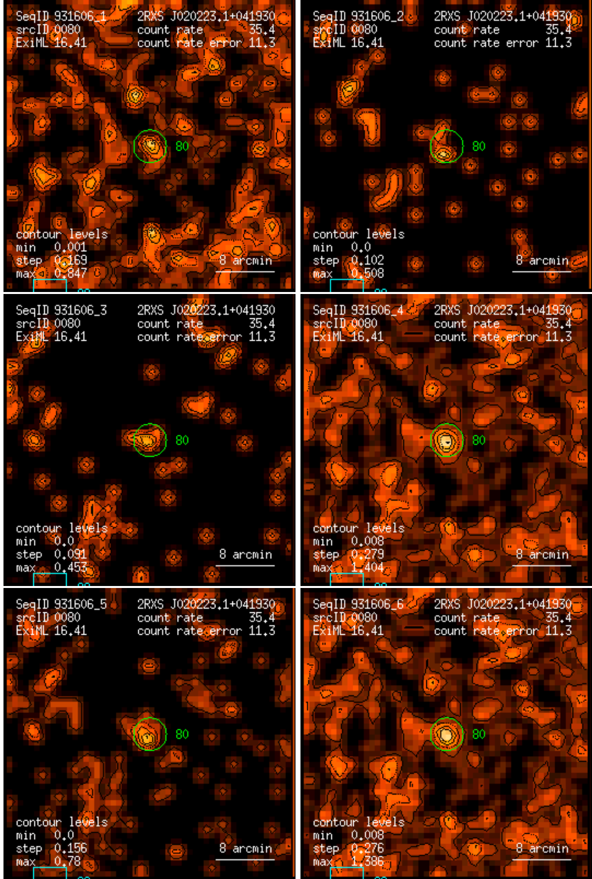
Figure 80: RASS 931606: detection 0080: band rate images, Gaussian filter: (1) PSPC channels 11 – 41, (2) 52 – 90, (3) 91 – 201, (4) 11 – 235, (5) 52 – 201, (6) 11 – 201. Broad band rates in counts/ks. Band rate contour levels in counts/ks/arcmin 2 .
