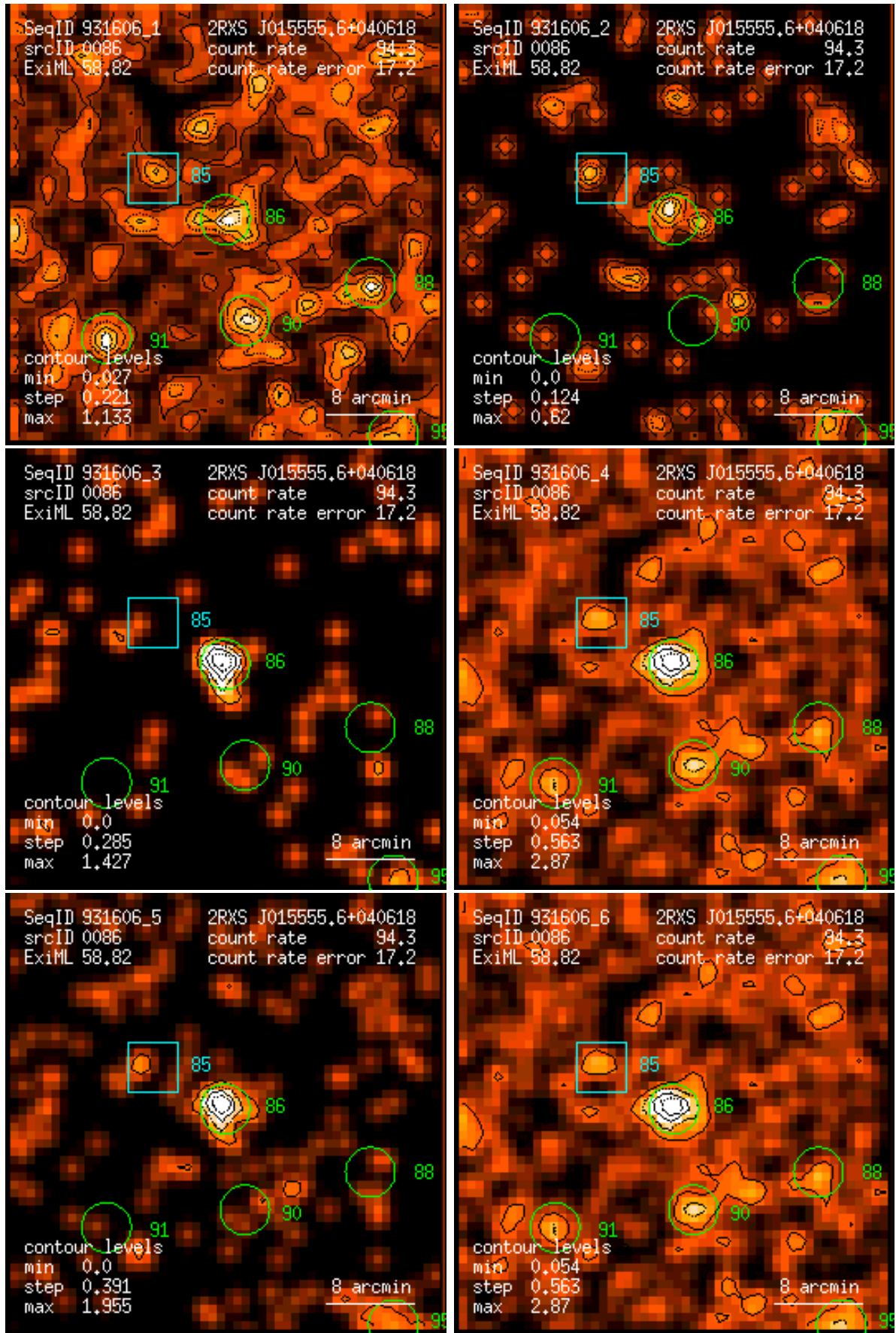
Figure 86: RASS 931606: detection 0086: band rate images, Gaussian filter: (1) PSPC channels 11 – 41, (2) 52 – 90, (3) 91 – 201, (4) 11 – 235, (5) 52 – 201, (6) 11 – 201. Broad band rates in counts/ks. Band rate contour levels in counts/ks/arcmin 2 .
