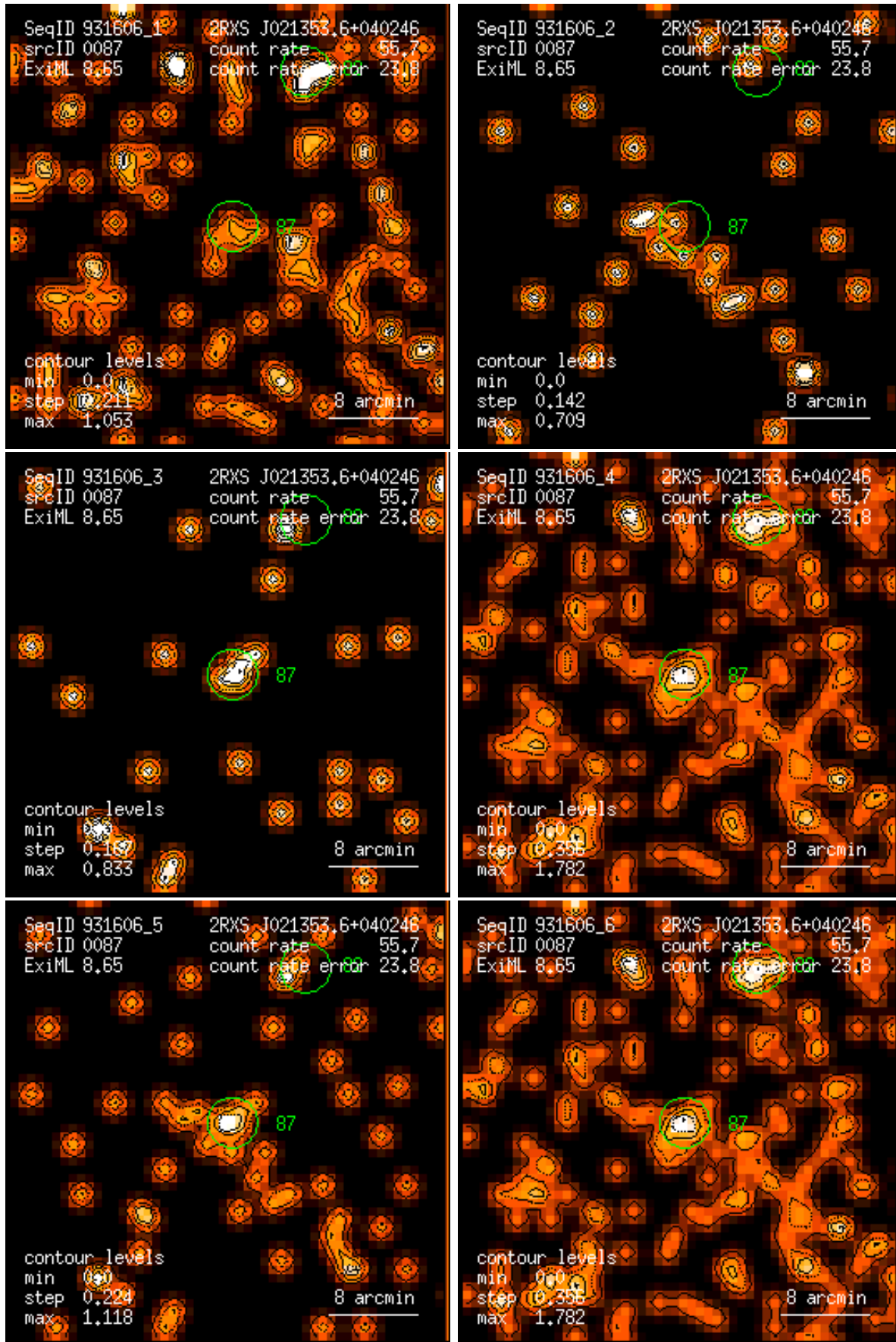
Figure 87: RASS 931606: detection 0087: band rate images, Gaussian filter: (1) PSPC channels 11 – 41, (2) 52 – 90, (3) 91 – 201, (4) 11 – 235, (5) 52 – 201, (6) 11 – 201. Broad band rates in counts/ks. Band rate contour levels in counts/ks/arcmin 2 .
