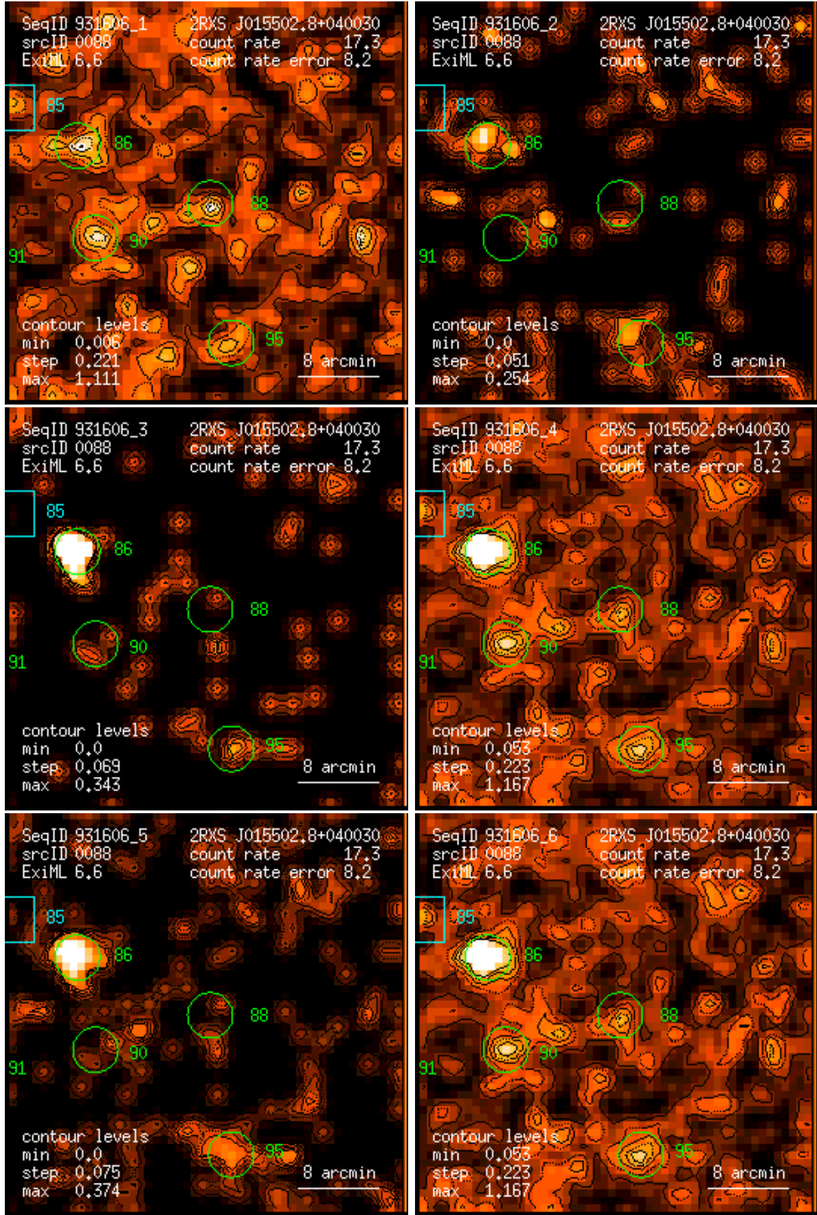
Figure 88: RASS 931606: detection 0088: band rate images, Gaussian filter: (1) PSPC channels 11 – 41, (2) 52 – 90, (3) 91 – 201, (4) 11 – 235, (5) 52 – 201, (6) 11 – 201. Broad band rates in counts/ks. Band rate contour levels in counts/ks/arcmin 2 .
