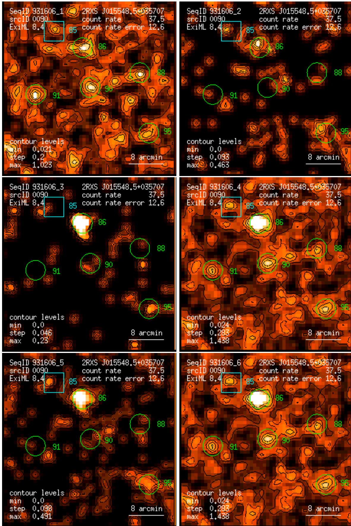
Figure 90: RASS 931606: detection 0090: band rate images, Gaussian filter: (1) PSPC channels 11 – 41, (2) 52 – 90, (3) 91 – 201, (4) 11 – 235, (5) 52 – 201, (6) 11 – 201. Broad band rates in counts/ks. Band rate contour levels in counts/ks/arcmin 2 .
