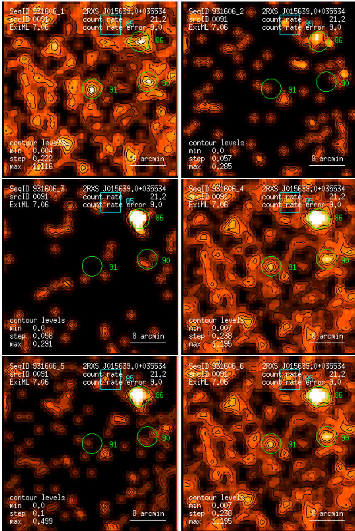
Figure 91: RASS 931606: detection 0091: band rate images, Gaussian filter: (1) PSPC channels 11 – 41, (2) 52 – 90, (3) 91 – 201, (4) 11 – 235, (5) 52 – 201, (6) 11 – 201. Broad band rates in counts/ks. Band rate contour levels in counts/ks/arcmin 2 .
