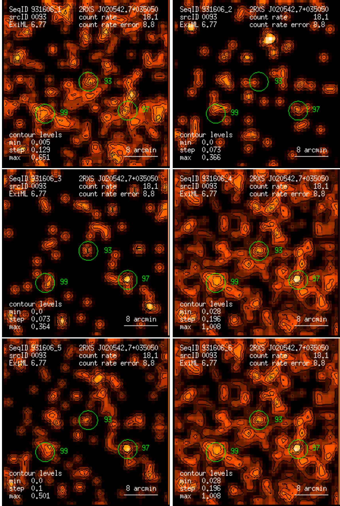
Figure 93: RASS 931606: detection 0093: band rate images, Gaussian filter: (1) PSPC channels 11 – 41, (2) 52 – 90, (3) 91 – 201, (4) 11 – 235, (5) 52 – 201, (6) 11 – 201. Broad band rates in counts/ks. Band rate contour levels in counts/ks/arcmin 2 .
