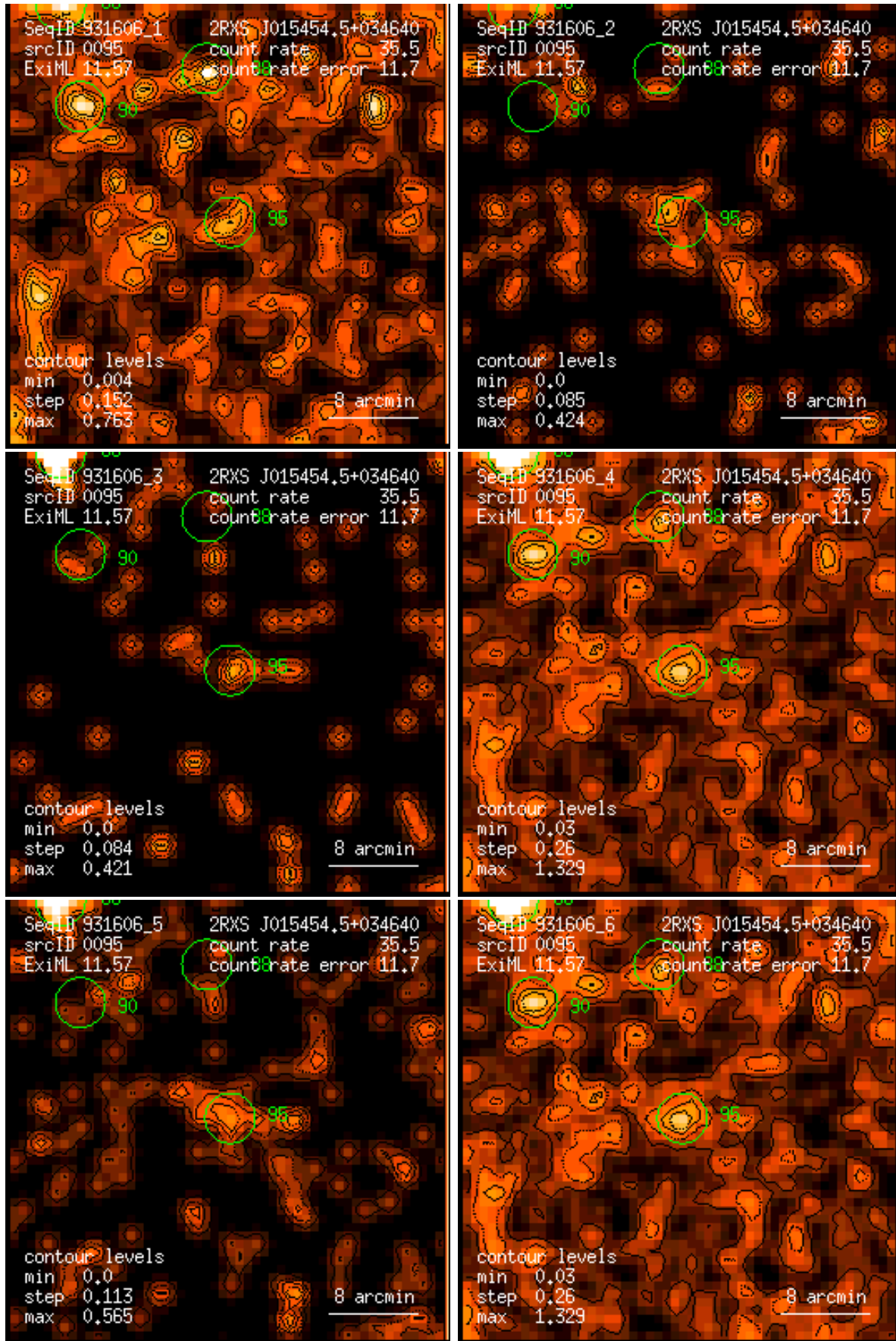
Figure 95: RASS 931606: detection 0095: band rate images, Gaussian filter: (1) PSPC channels 11 – 41, (2) 52 – 90, (3) 91 – 201, (4) 11 – 235, (5) 52 – 201, (6) 11 – 201. Broad band rates in counts/ks. Band rate contour levels in counts/ks/arcmin 2 .
