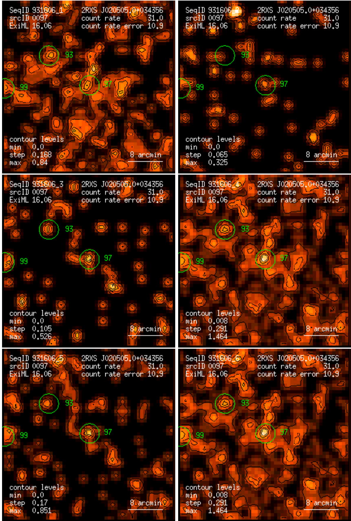
Figure 97: RASS 931606: detection 0097: band rate images, Gaussian filter: (1) PSPC channels 11 – 41, (2) 52 – 90, (3) 91 – 201, (4) 11 – 235, (5) 52 – 201, (6) 11 – 201. Broad band rates in counts/ks. Band rate contour levels in counts/ks/arcmin 2 .
