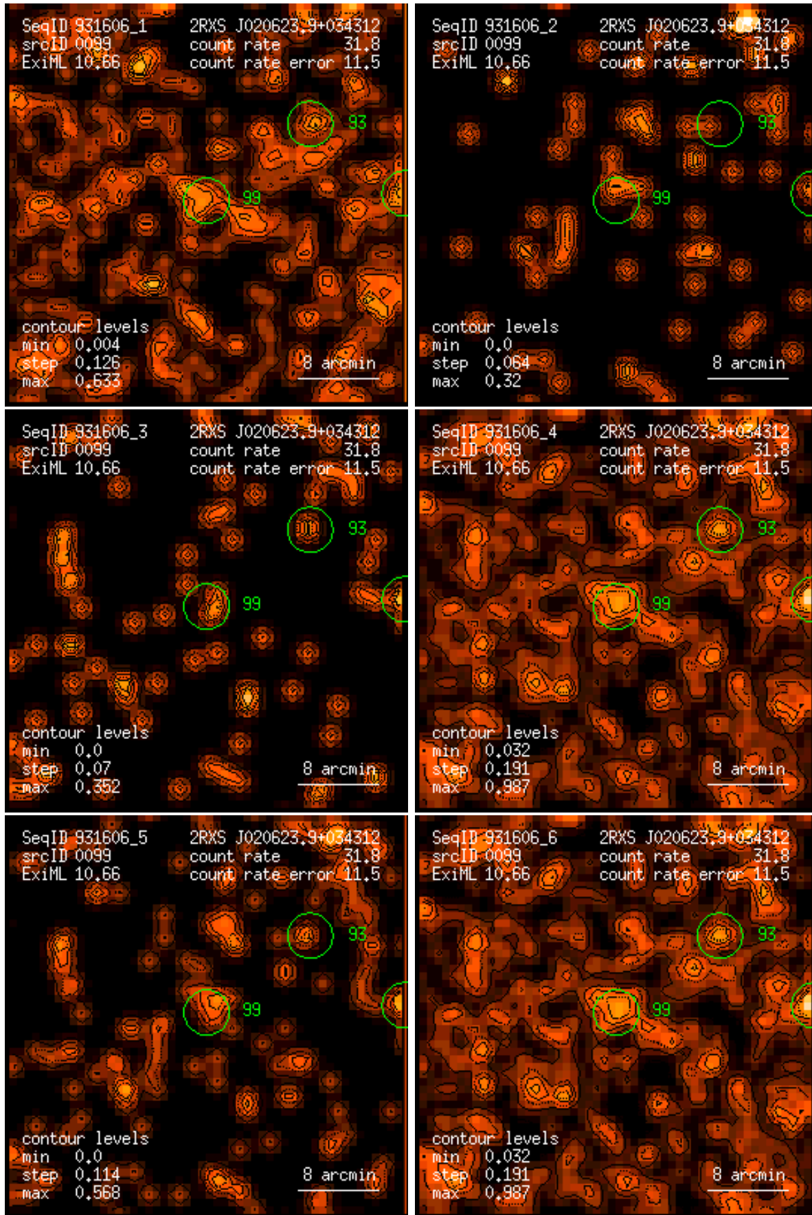
Figure 99: RASS 931606: detection 0099: band rate images, Gaussian filter: (1) PSPC channels 11 – 41, (2) 52 – 90, (3) 91 – 201, (4) 11 – 235, (5) 52 – 201, (6) 11 – 201. Broad band rates in counts/ks. Band rate contour levels in counts/ks/arcmin 2 .
