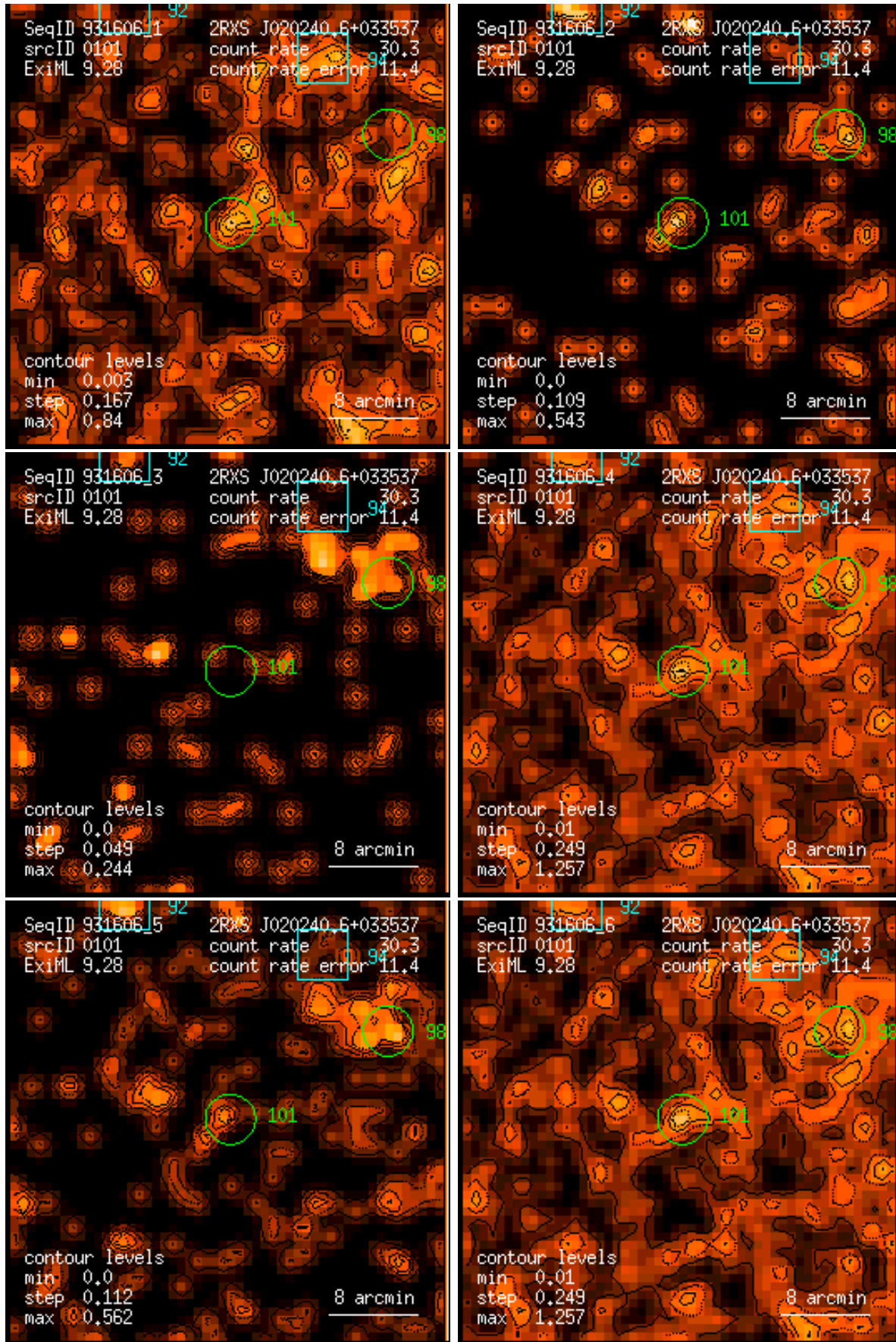
Figure 101: RASS 931606: detection 0101: band rate images, Gaussian filter: (1) PSPC channels 11 – 41, (2) 52 – 90, (3) 91 – 201, (4) 11 – 235, (5) 52 – 201, (6) 11 – 201. Broad band rates in counts/ks. Band rate contour levels in counts/ks/arcmin 2 .
