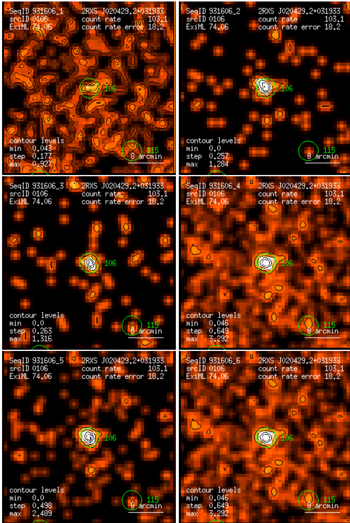
Figure 106: RASS 931606: detection 0106: band rate images, Gaussian filter: (1) PSPC channels 11 – 41, (2) 52 – 90, (3) 91 – 201, (4) 11 – 235, (5) 52 – 201, (6) 11 – 201. Broad band rates in counts/ks. Band rate contour levels in counts/ks/arcmin 2 .
