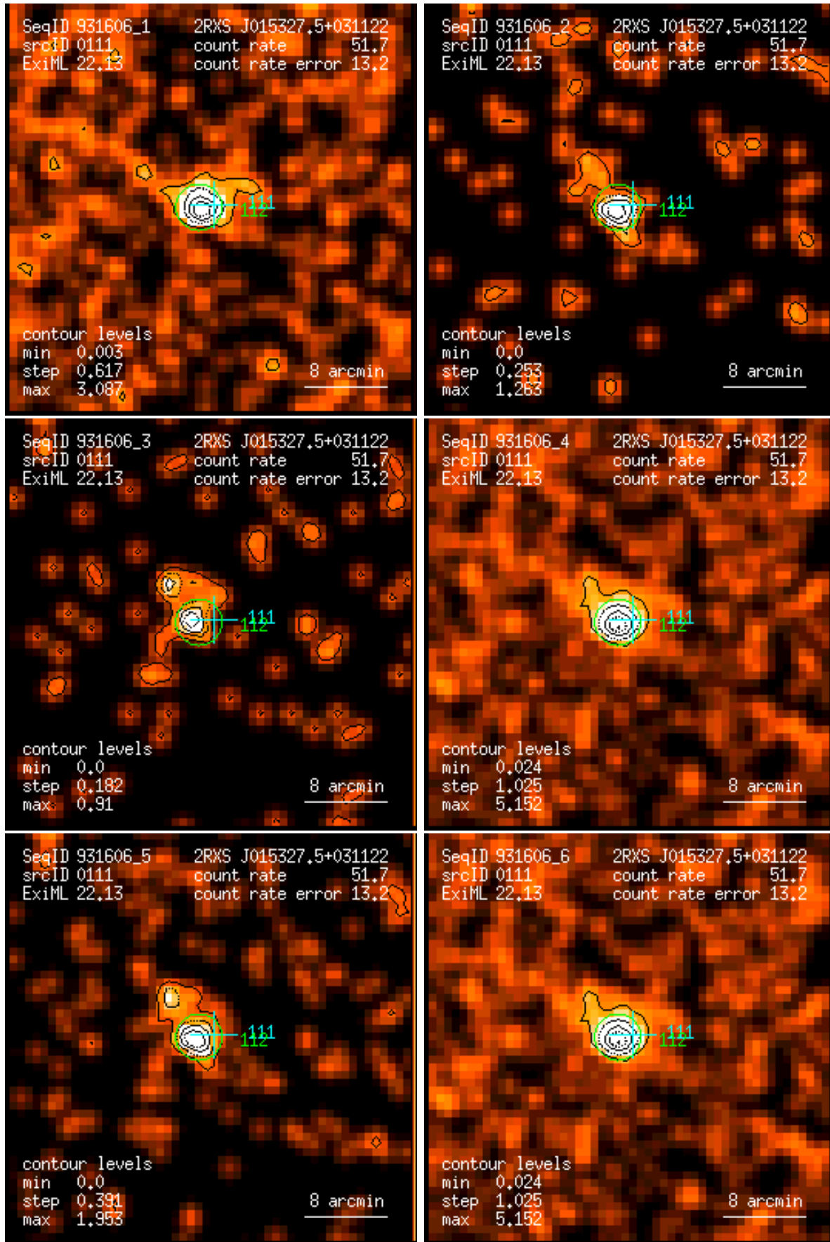
Figure 111: RASS 931606: detection 0111: band rate images, Gaussian filter: (1) PSPC channels 11 – 41, (2) 52 – 90, (3) 91 – 201, (4) 11 – 235, (5) 52 – 201, (6) 11 – 201. Broad band rates in counts/ks. Band rate contour levels in counts/ks/arcmin 2 .
