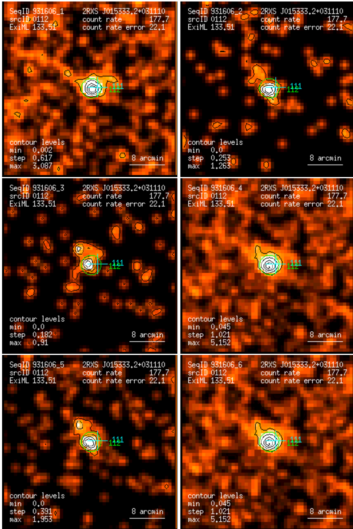
Figure 112: RASS 931606: detection 0112: band rate images, Gaussian filter: (1) PSPC channels 11 – 41, (2) 52 – 90, (3) 91 – 201, (4) 11 – 235, (5) 52 – 201, (6) 11 – 201. Broad band rates in counts/ks. Band rate contour levels in counts/ks/arcmin 2 .
