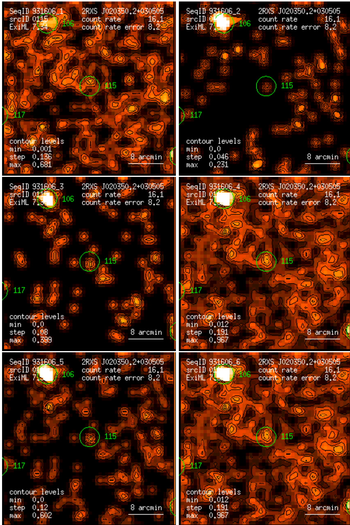
Figure 115: RASS 931606: detection 0115: band rate images, Gaussian filter: (1) PSPC channels 11 – 41, (2) 52 – 90, (3) 91 – 201, (4) 11 – 235, (5) 52 – 201, (6) 11 – 201. Broad band rates in counts/ks. Band rate contour levels in counts/ks/arcmin 2 .
