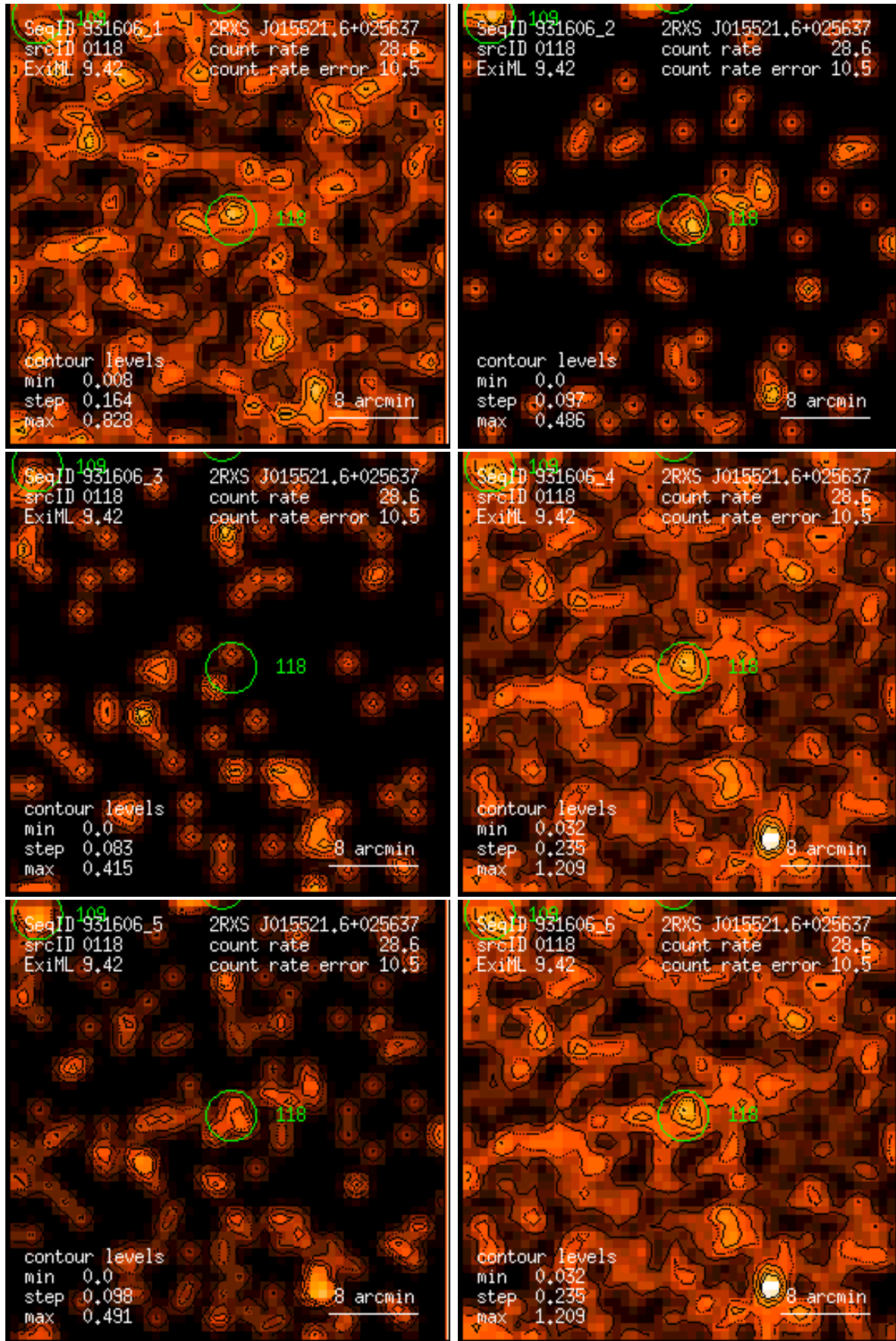
Figure 118: RASS 931606: detection 0118: band rate images, Gaussian filter: (1) PSPC channels 11 – 41, (2) 52 – 90, (3) 91 – 201, (4) 11 – 235, (5) 52 – 201, (6) 11 – 201. Broad band rates in counts/ks. Band rate contour levels in counts/ks/arcmin 2 .
